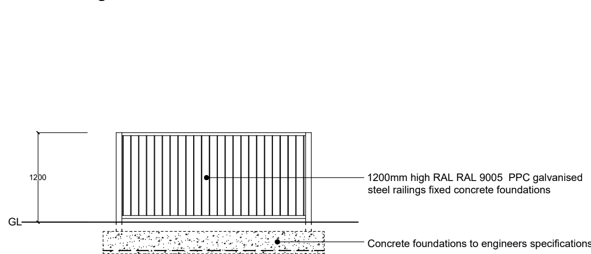
Metal Railings
