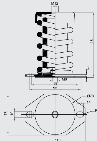
Dimensions AM-150 to AM-550
