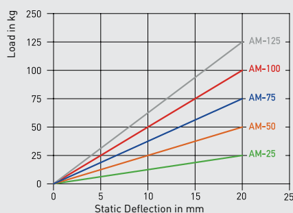
Static Deflection AM-25M to 125M
