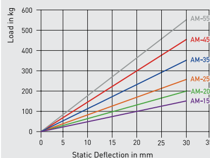
Static Deflection AM-150M to 550M
