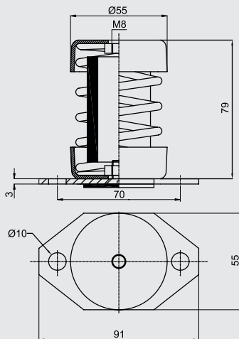
Dimensions AM-25 to AM-125
