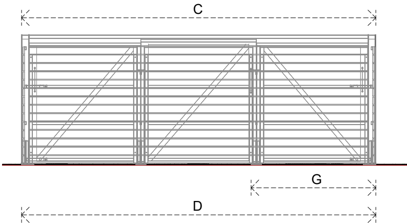
Front View - 1:50
