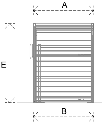
Side View - 1:50
