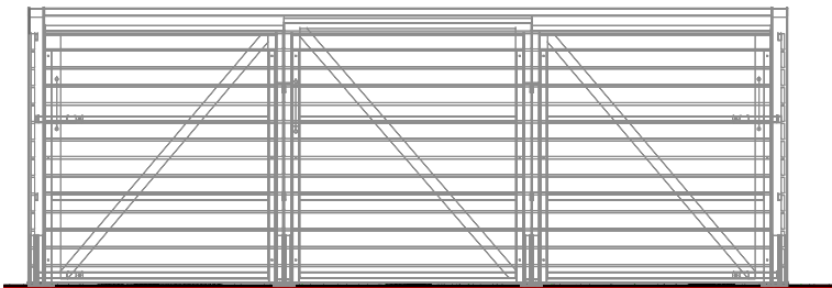
Rear View - 1:50
