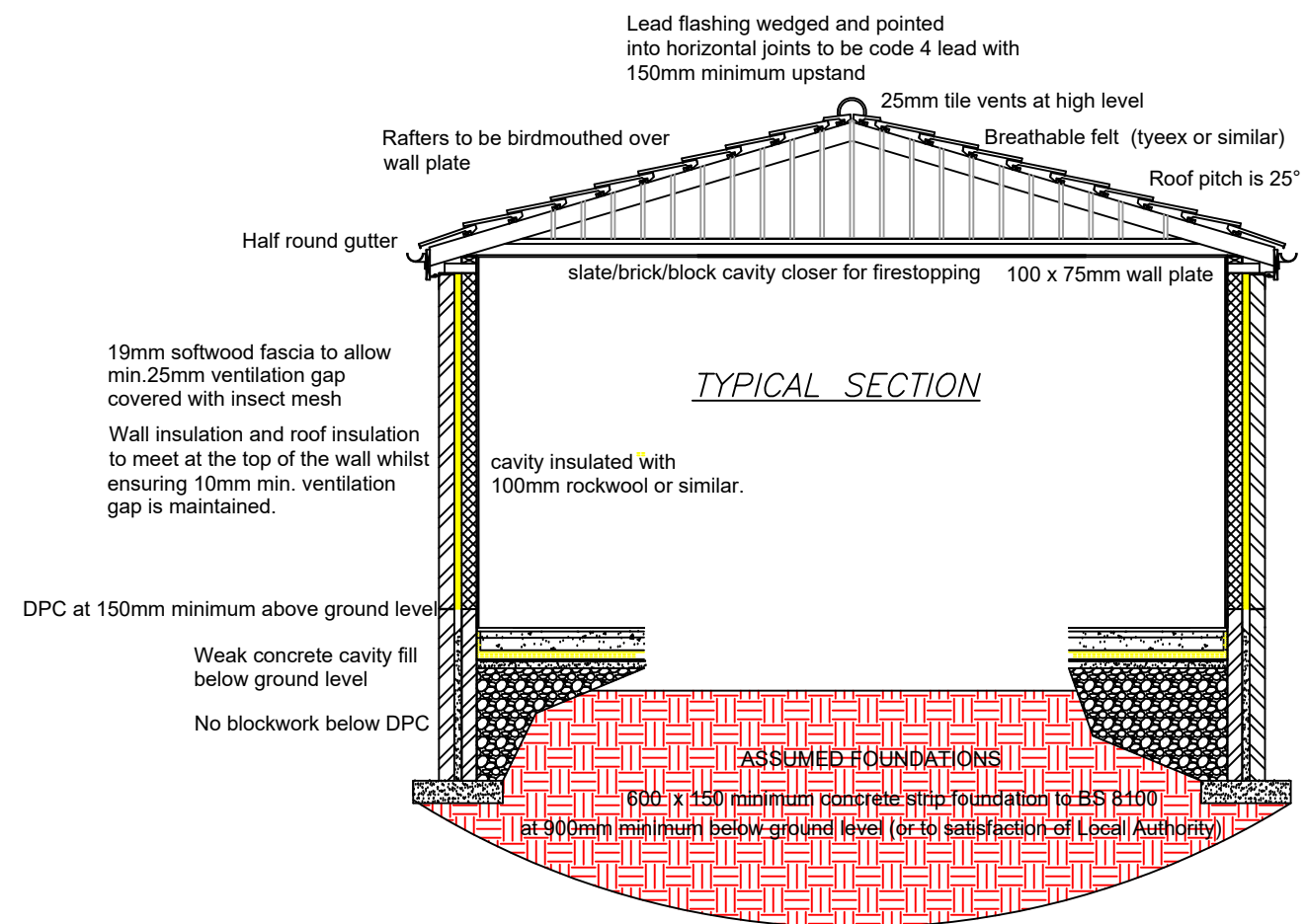
Roof & Typical Section - Ref : 008
