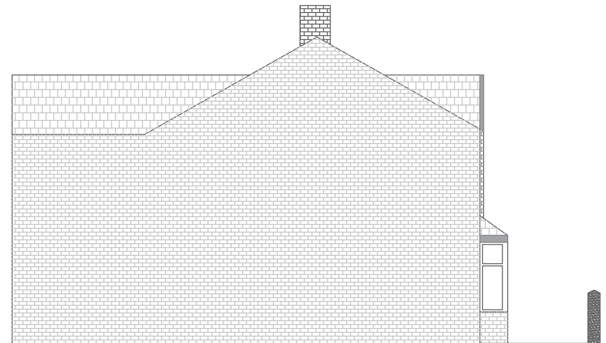
Existing L/H/S Elevation
