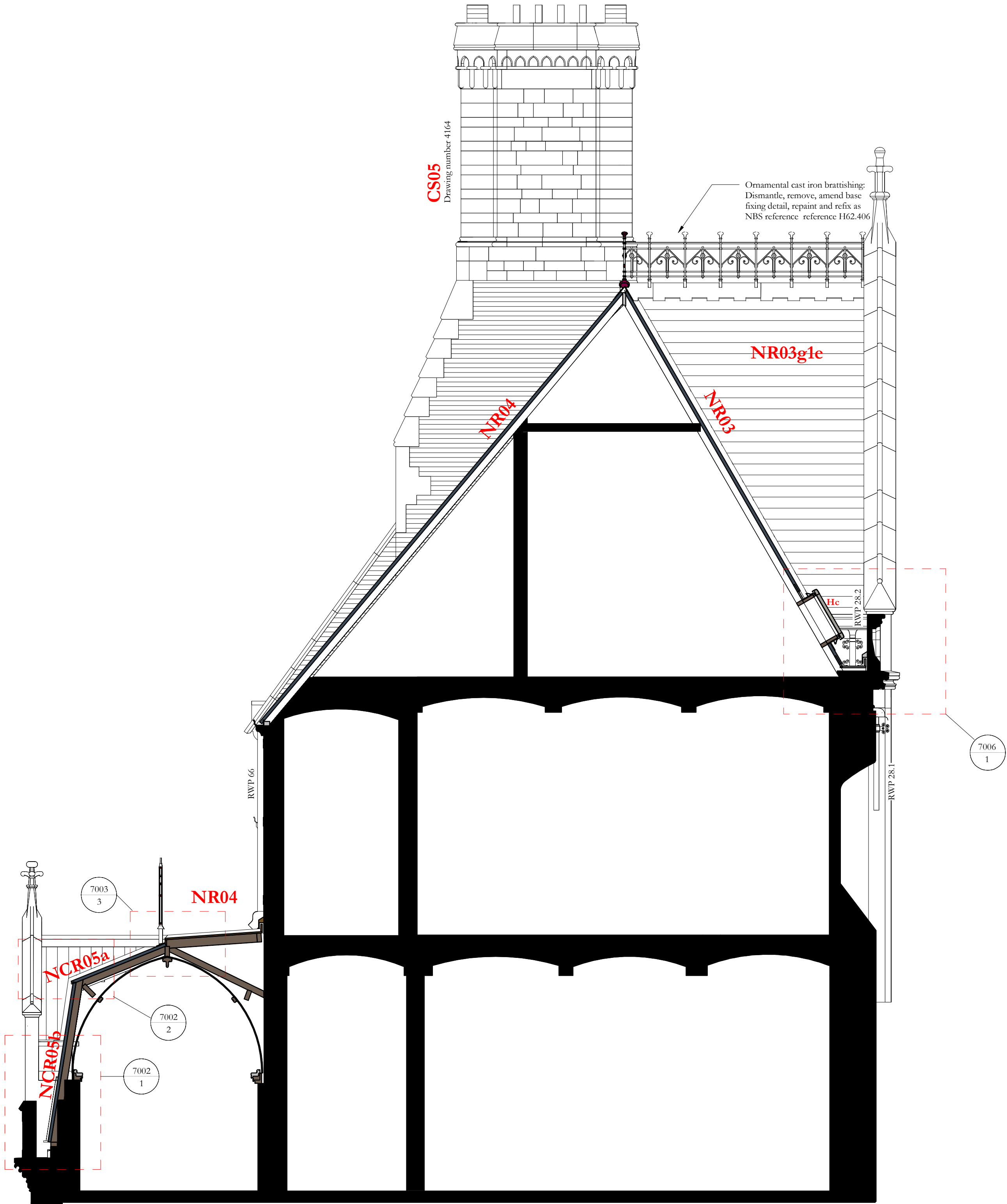
Section LL 1 : 50
