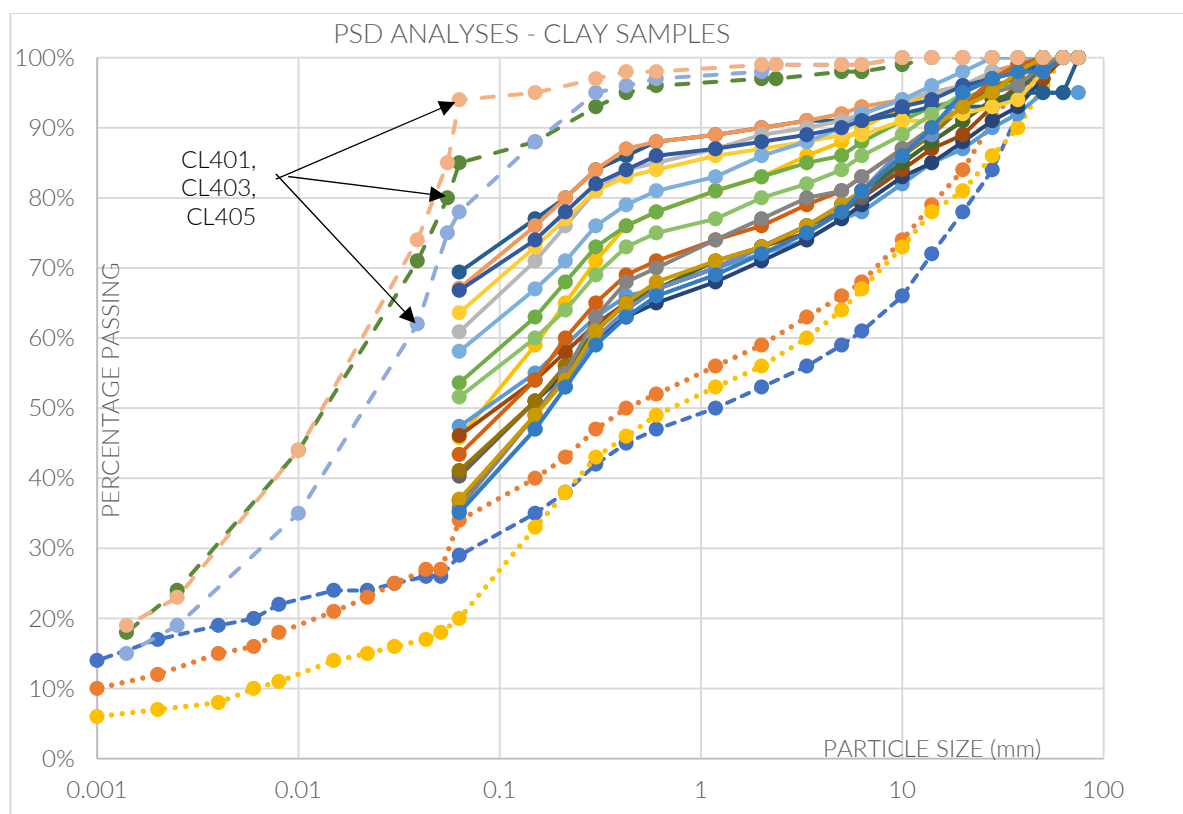
Figure 2 : PSD Analyses on Clay Made Ground
