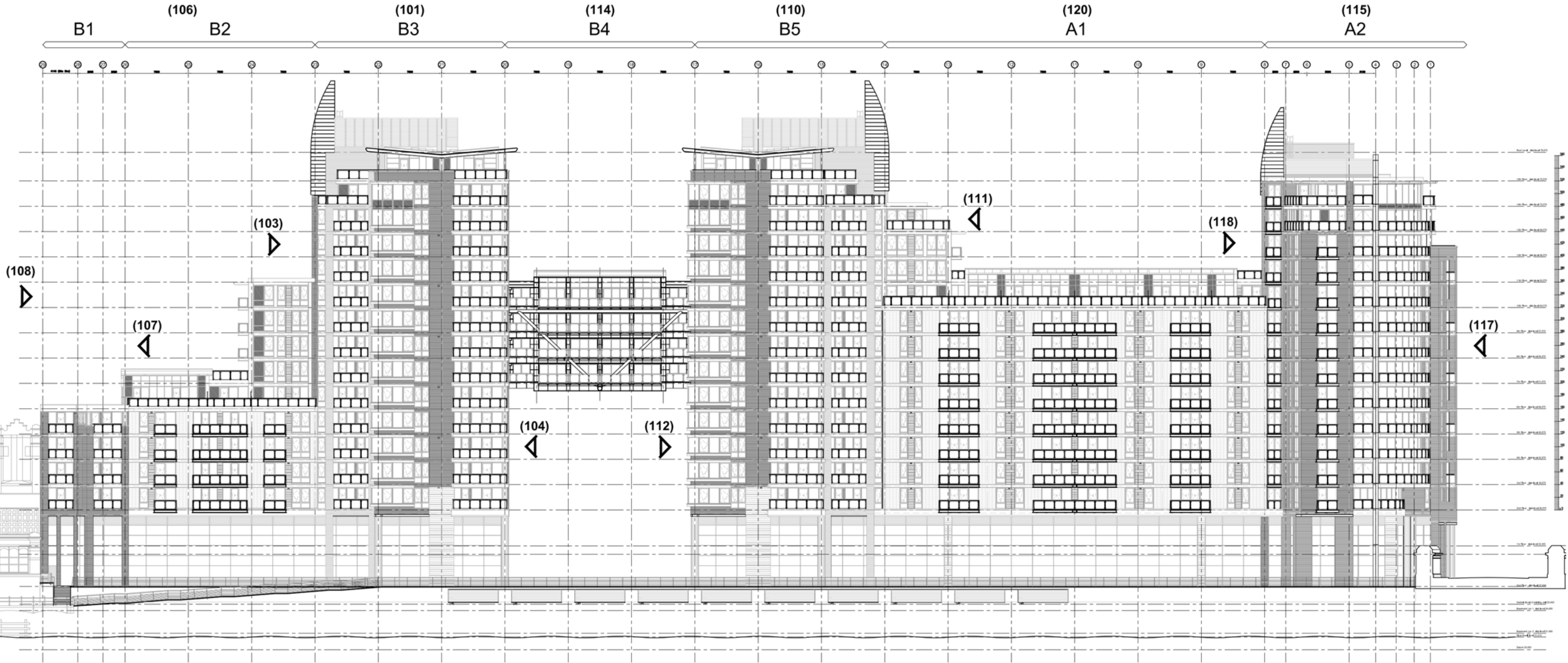
ELEVATION B - B RIVERSIDE
