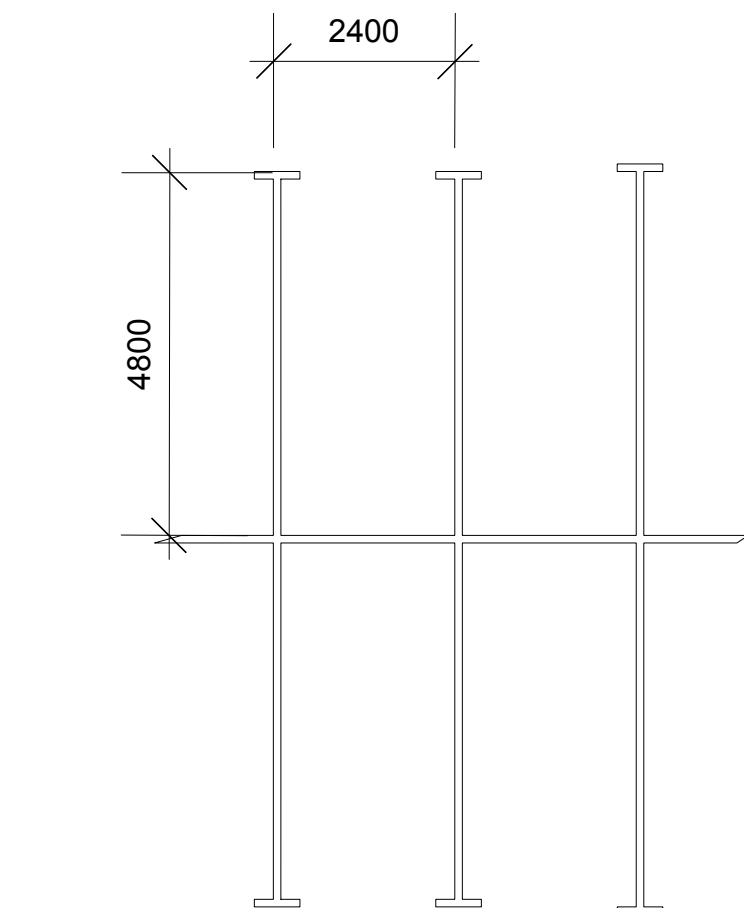
Detail - parking bay Lines 100mm wide. Thermoplastic White colour. Scale 1:100
