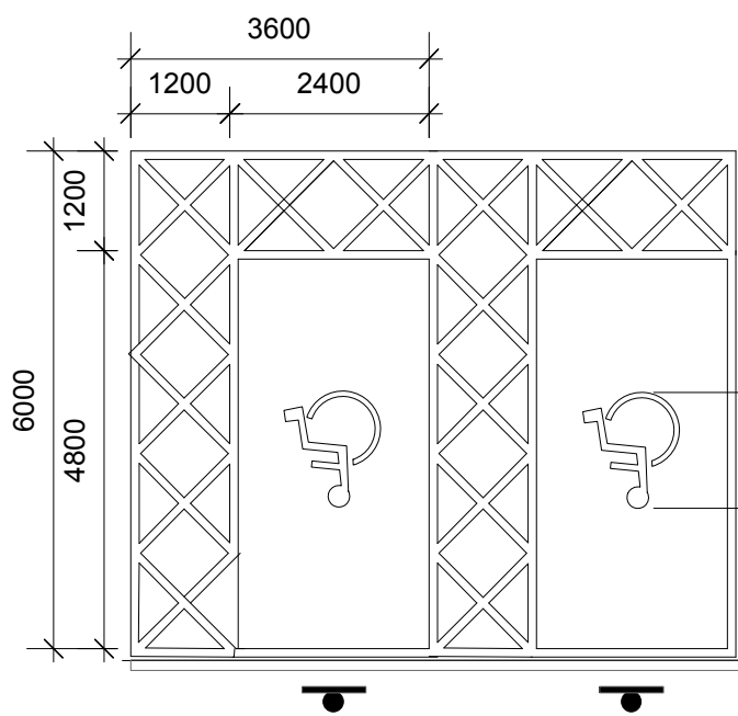
Accessibility parking sign Figure 3B-22 International symbol of accessible parking space set at kerb ends of bays. Lower edge set 1000mm above ground.
