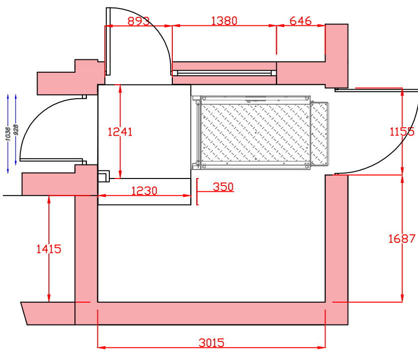
EXISTING PLAN LAYOUT
