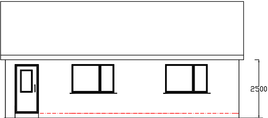
Front Elevation From 129
