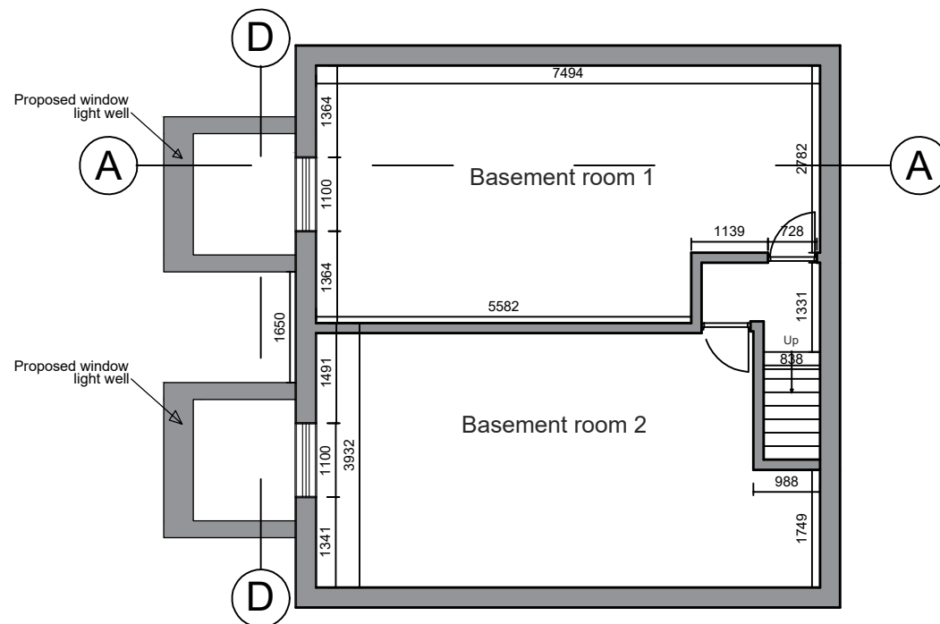
Proposed Basement
