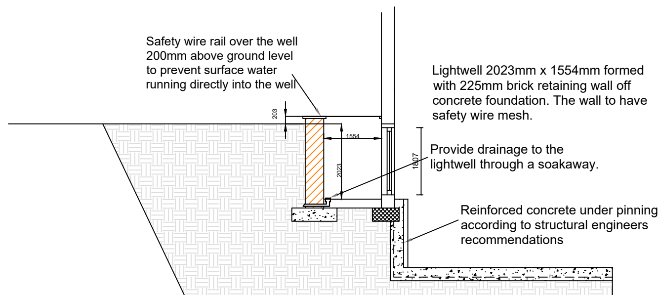
Section Through Lightwell Section AA
