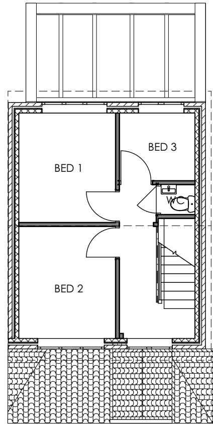
1. First Floor 1:100
