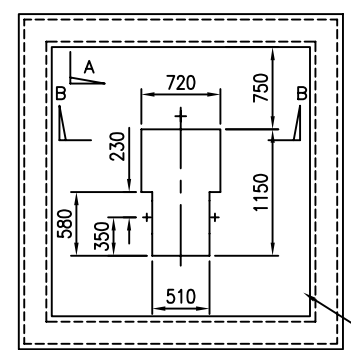
FOUNDATION PLAN
