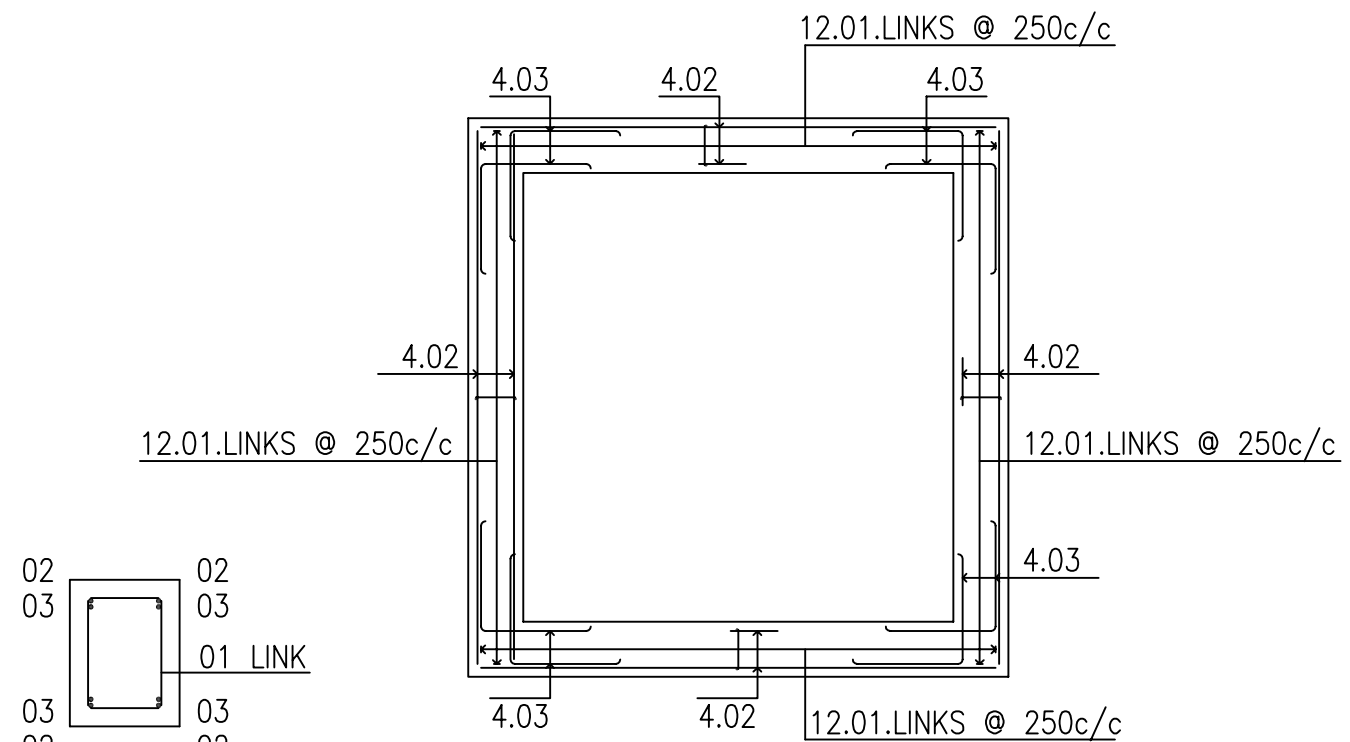
PLAN ON REINFORCED BEAM
