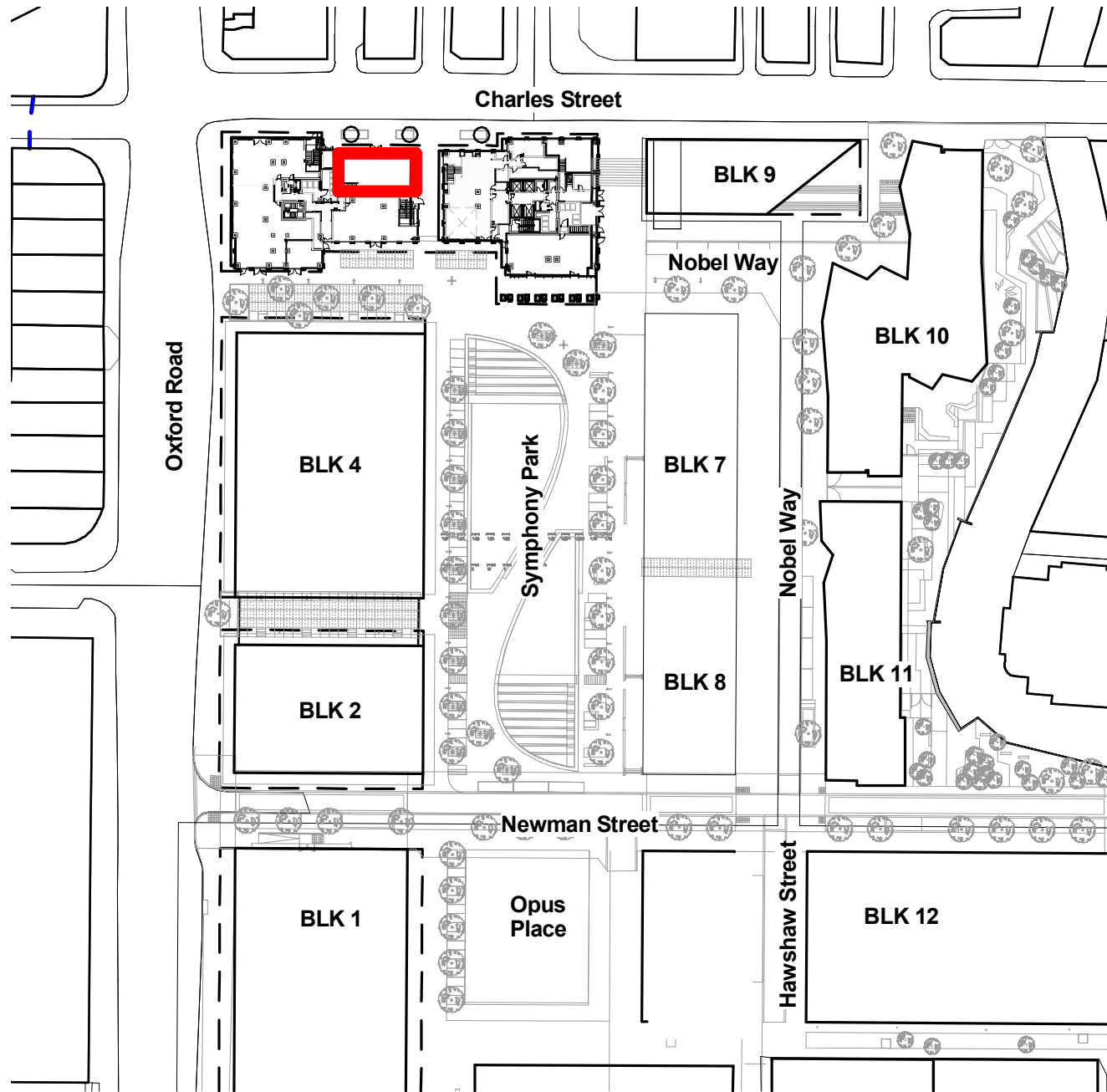
LOCATION PLAN 1:1250
