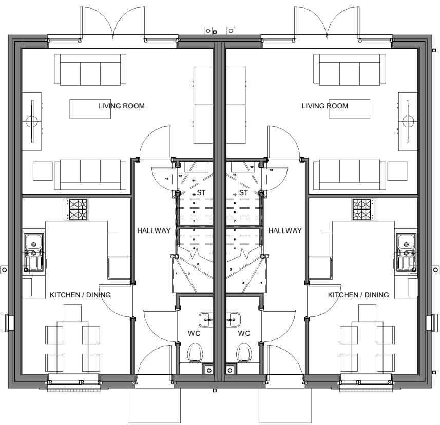
1 | HT D4 - 4B5P M4(1) - 00 PLAN 1 : 100
