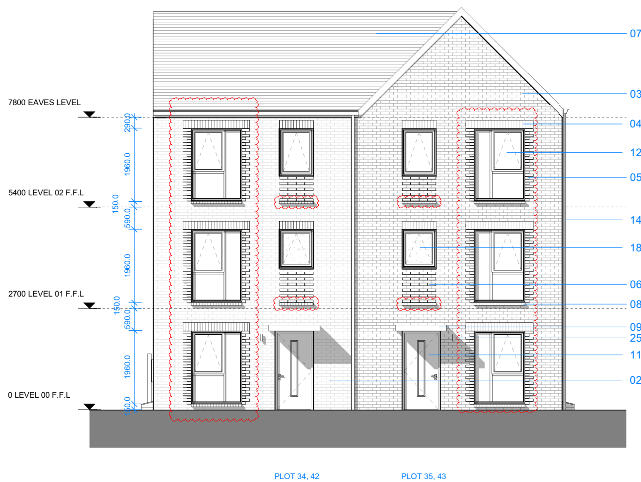
5 | HT D4 - 4B5P M4(1) - FRONT ELEVATION 1 : 100
