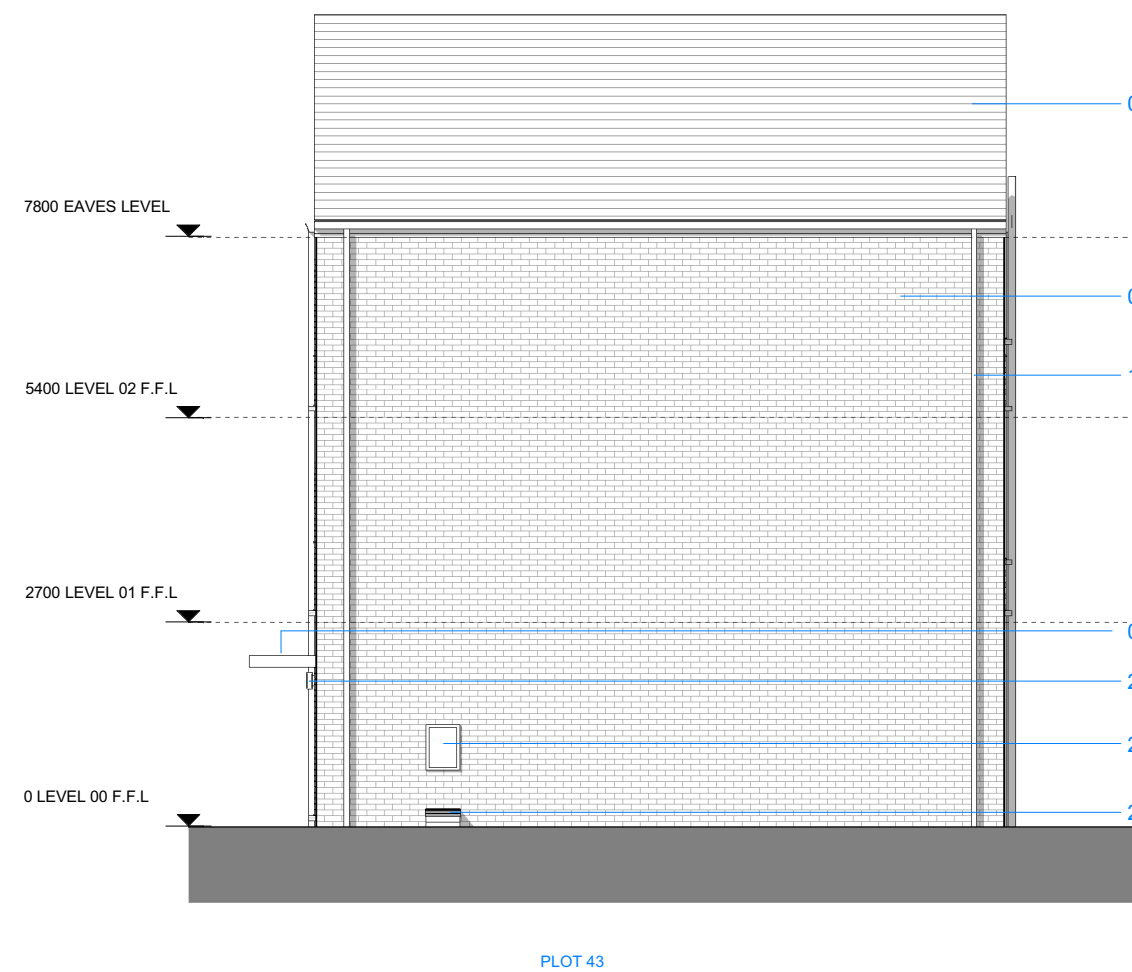
8 | HT D4 - 4B5P M4(1) - SIDE ELEVATION 02 1 : 100
