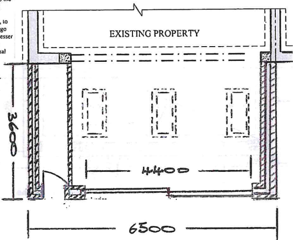
FOUNDATION / GROUND FLOOR LAYOUT
