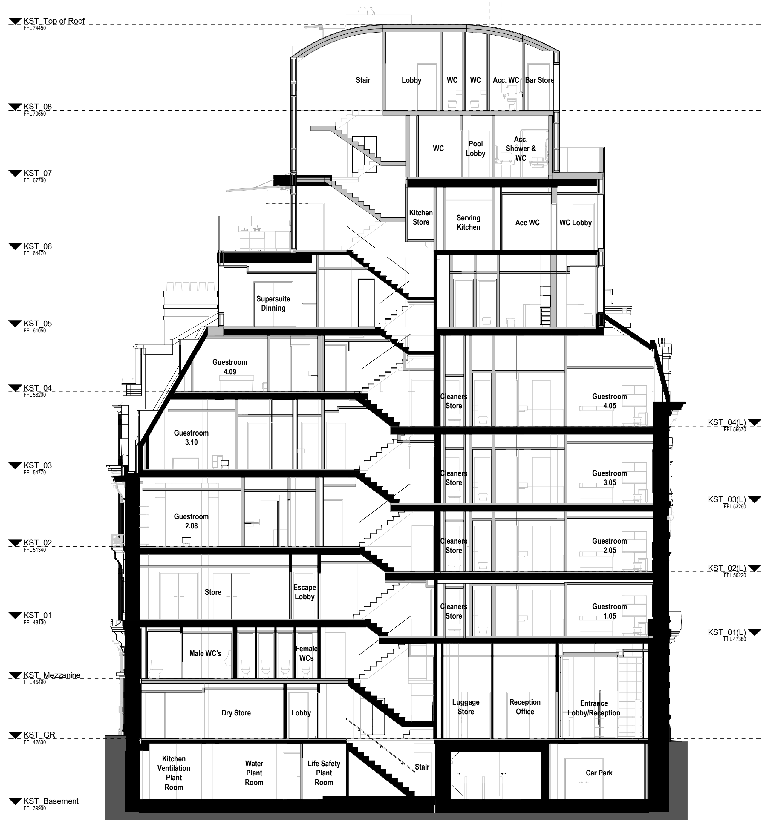
C Proposed Section CC 1:100
