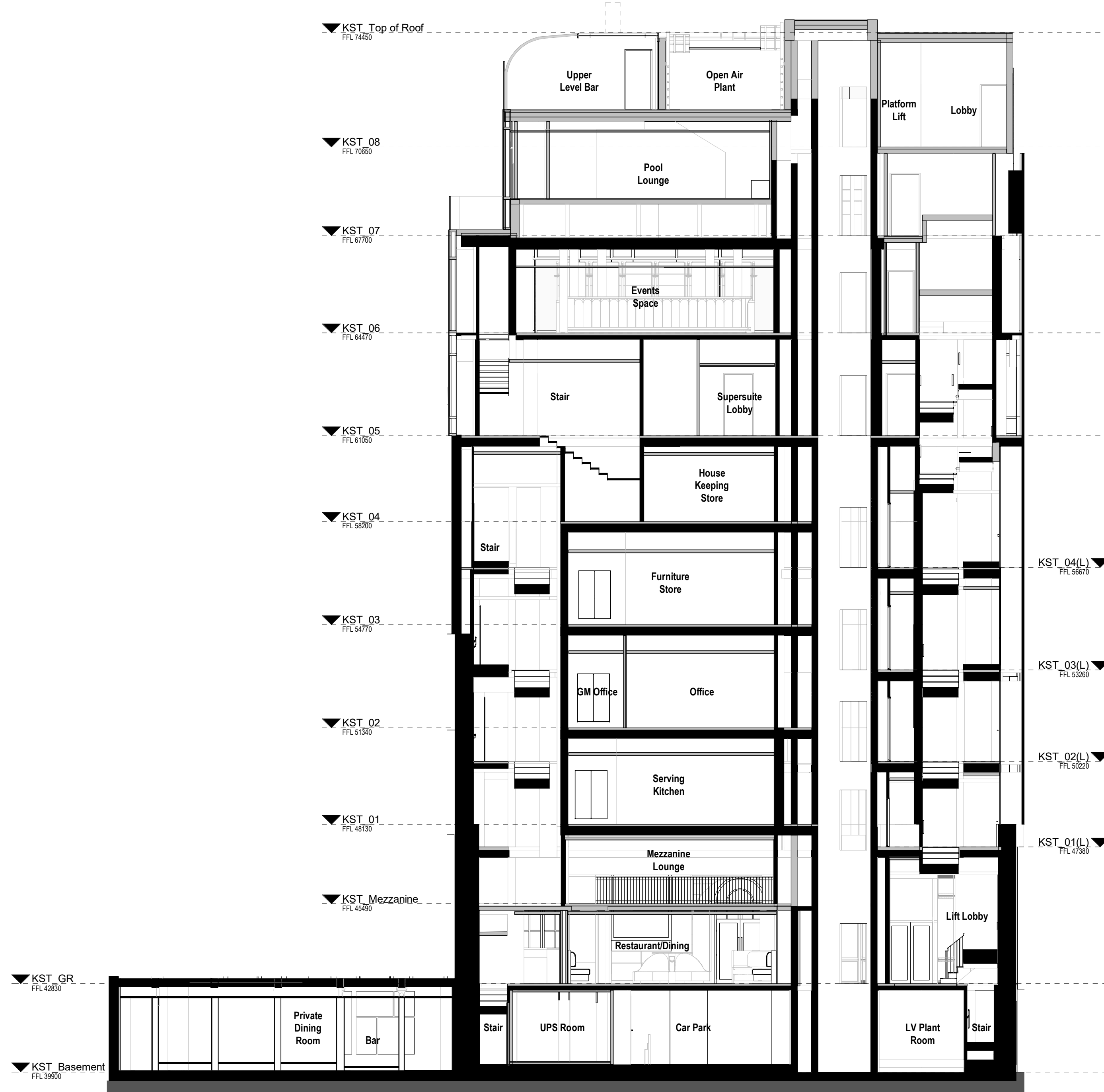
D Proposed Section DD 1:100
