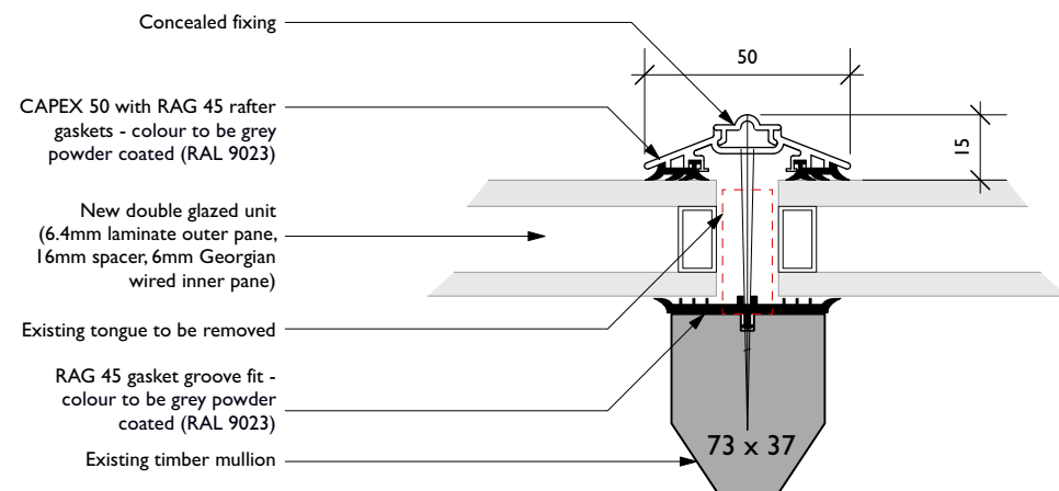
Detail 1 - Mullion detail
