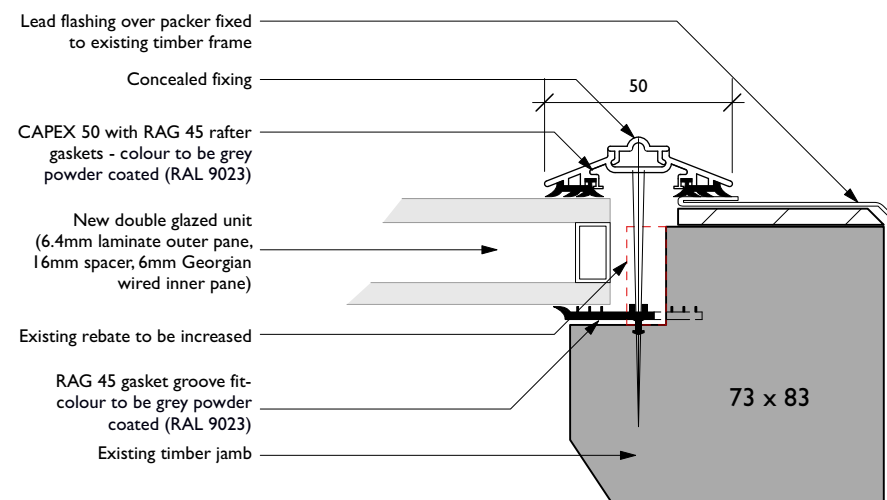
Detail 2 - Jamb detail
