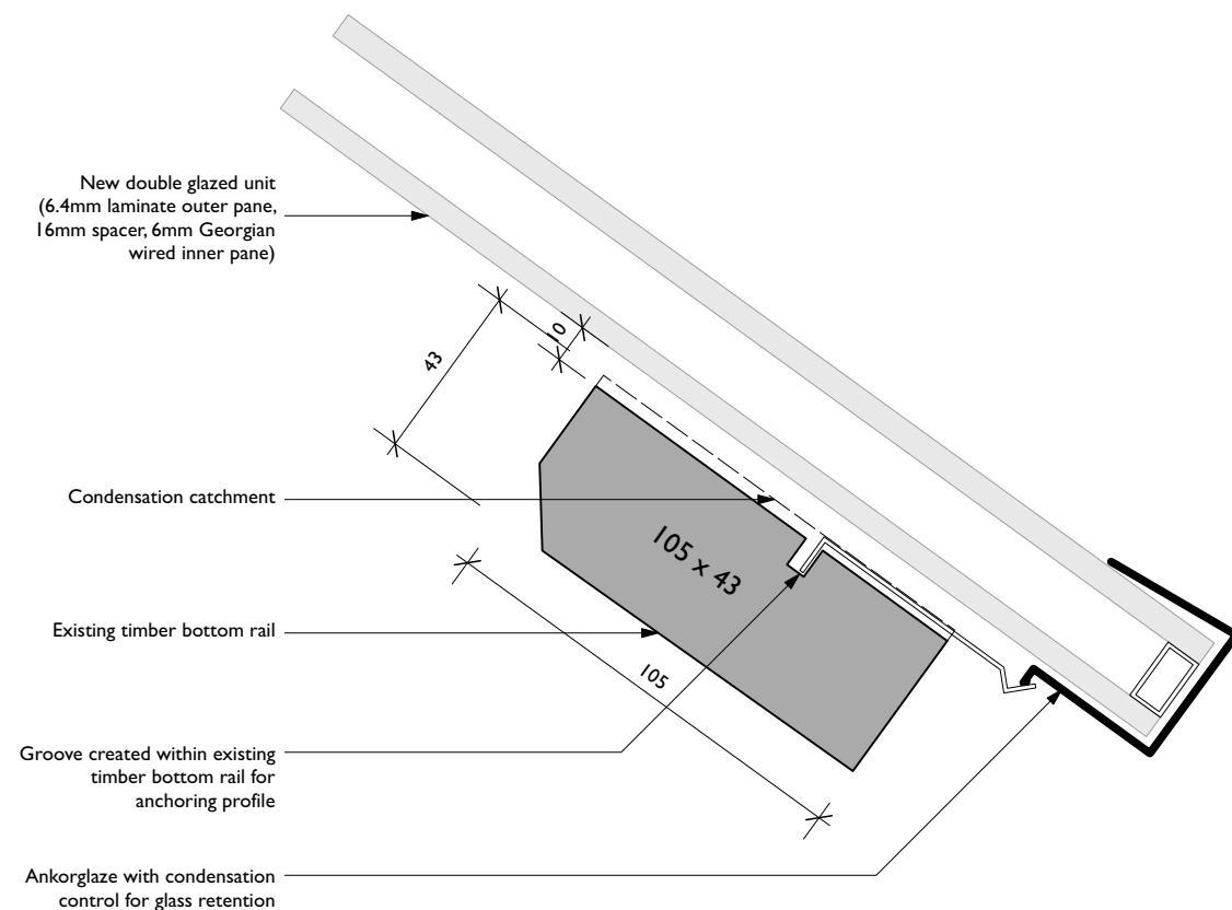
Detail 3 - Bottom Rail Detail
