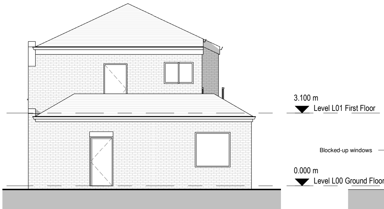
3 Existing North Elevation 1 : 100
