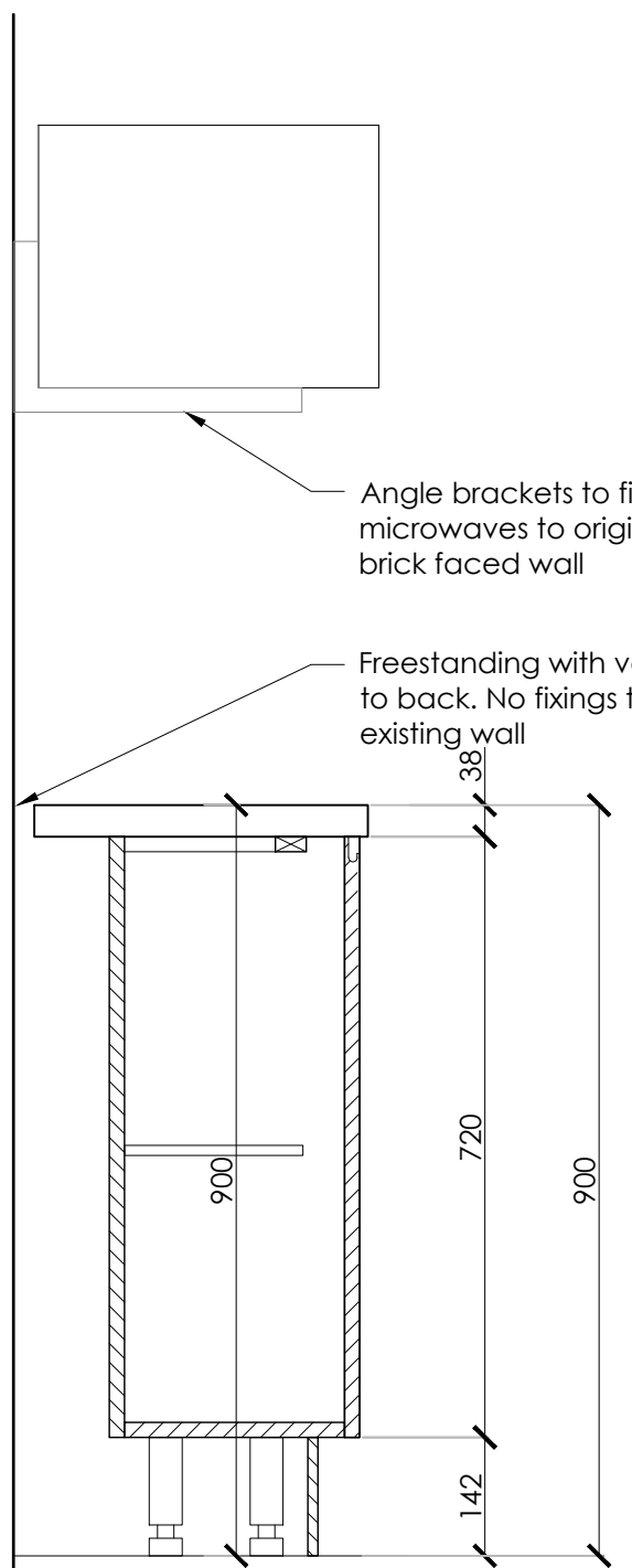
SECTION XX THROUGH FREE STANDING UNIT SCALE 1:10
