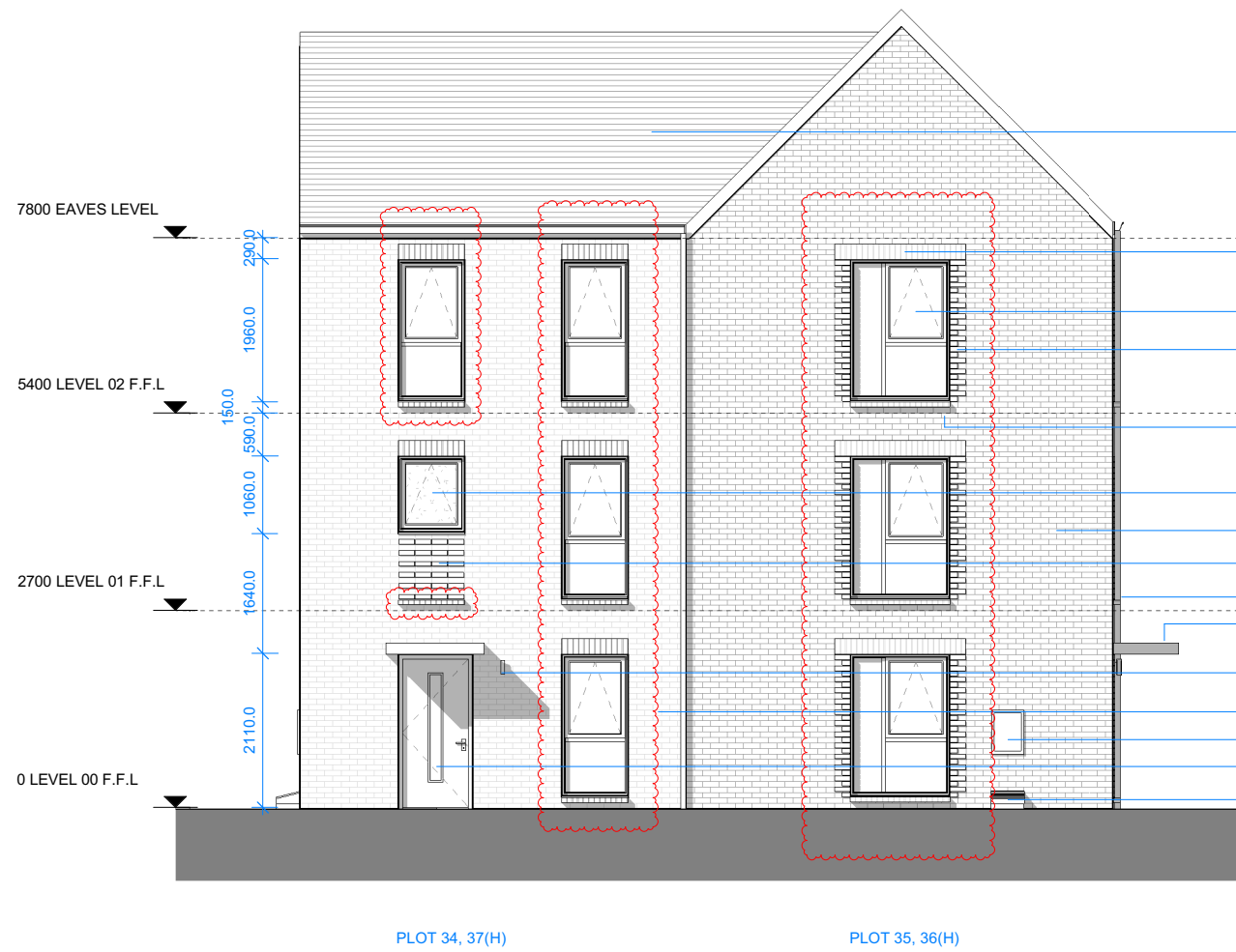
5 | HT D2 - 4B5P & 4B7P M4(1) - FRONT ELEVATION 1 : 100
