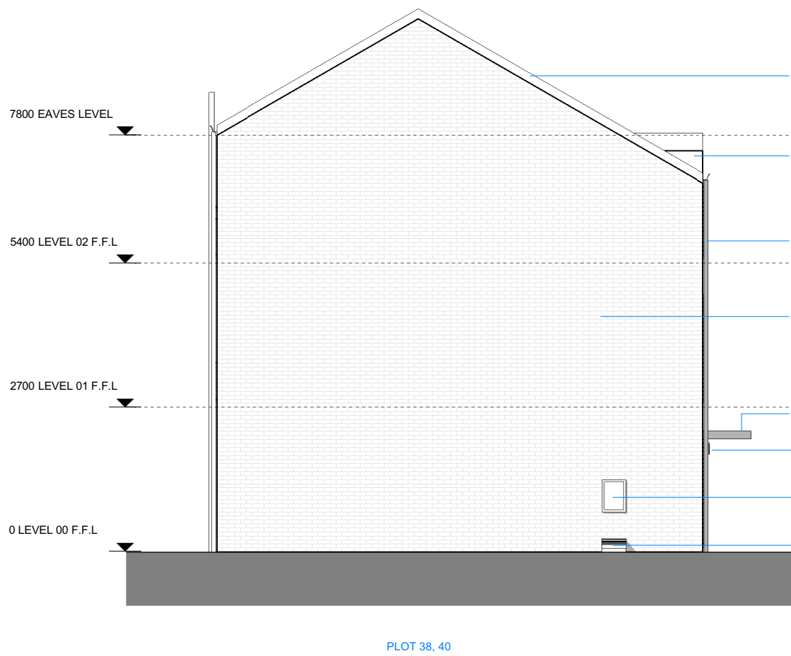
6 | HT D3 - 4B5P M4(1) - SIDE ELEVATION 01 1 : 100
