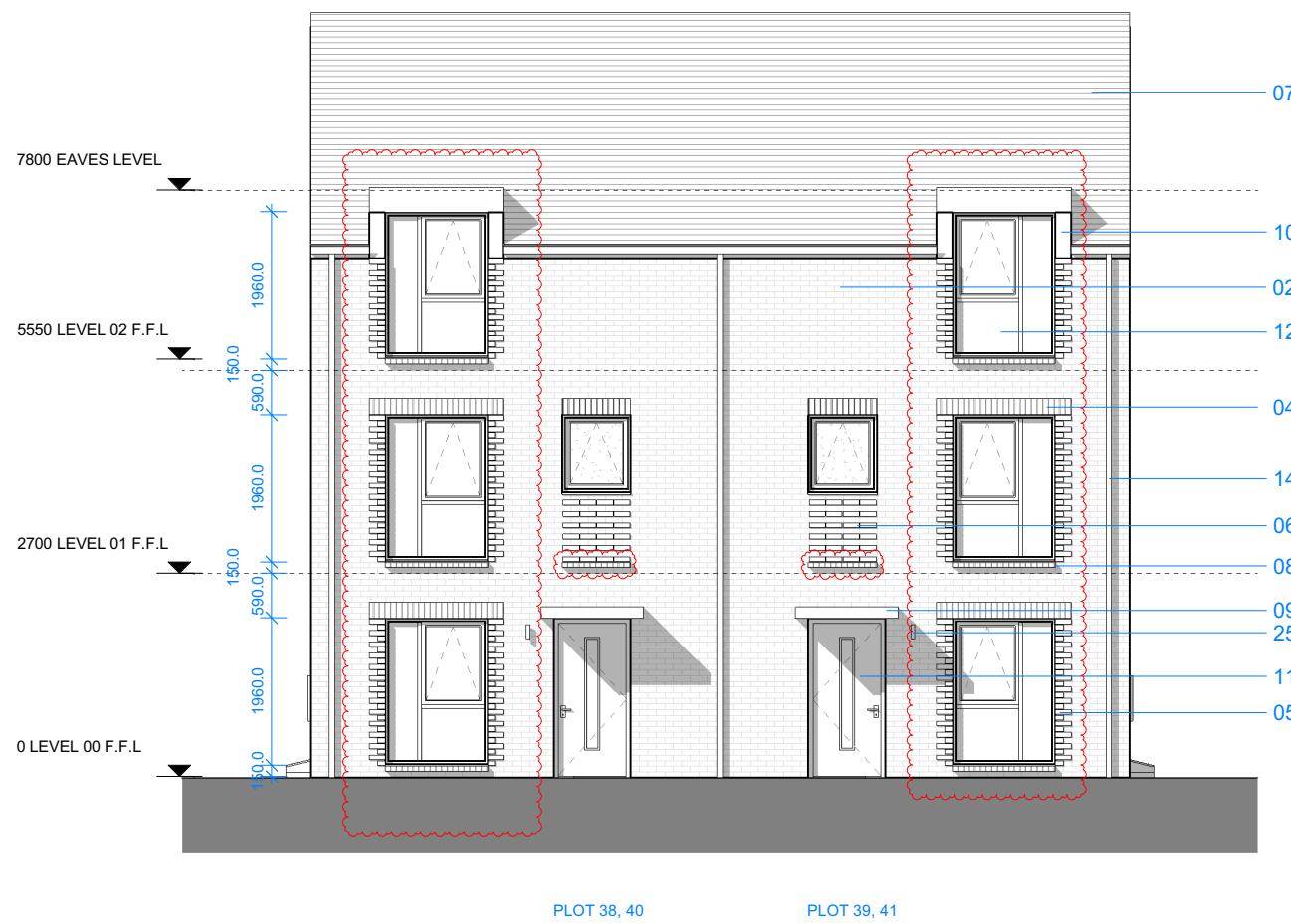
5 | HT D3 - 4B5P M4(1) - FRONT ELEVATION 1 : 100
