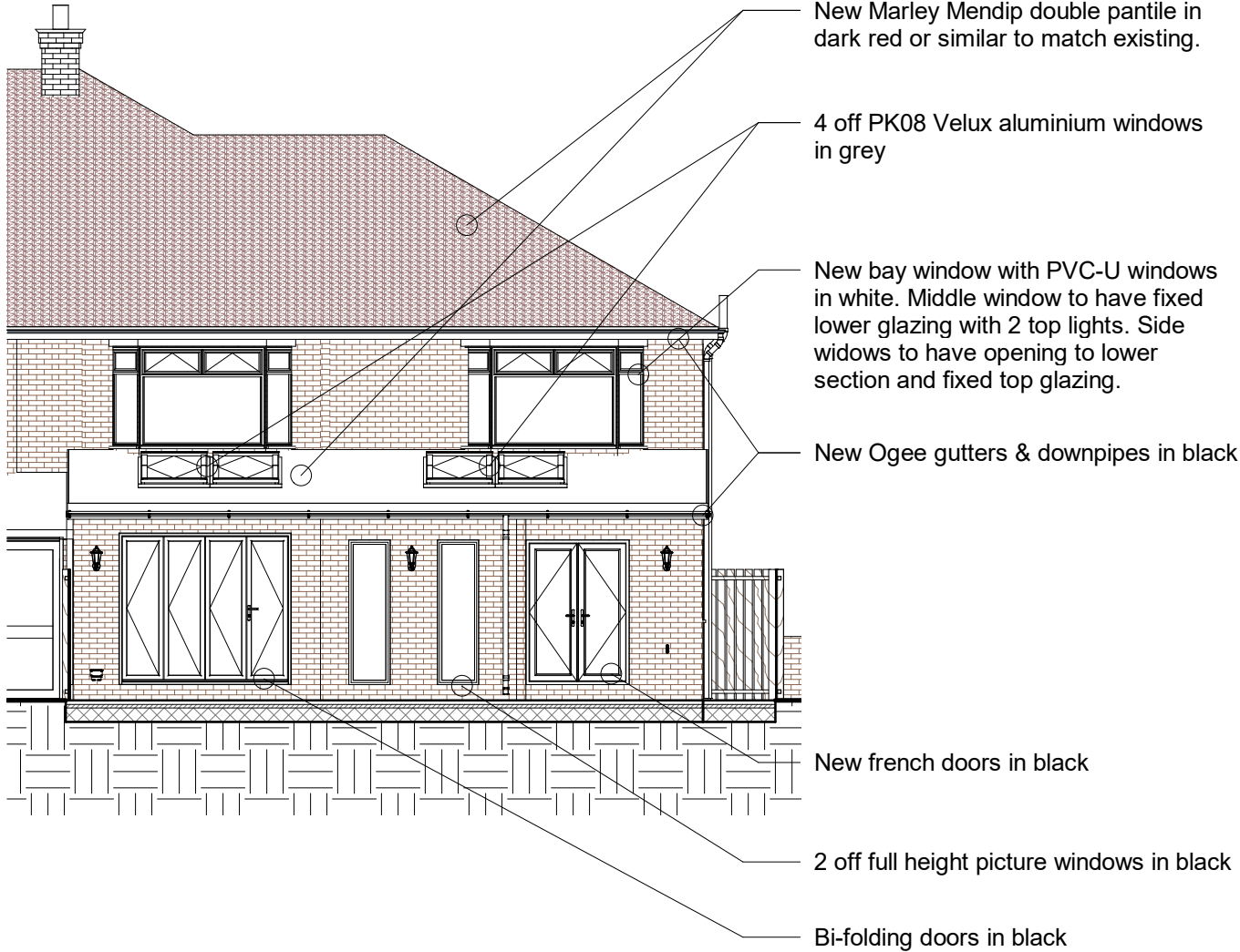
2 South Elevation - Proposed 1 : 100
