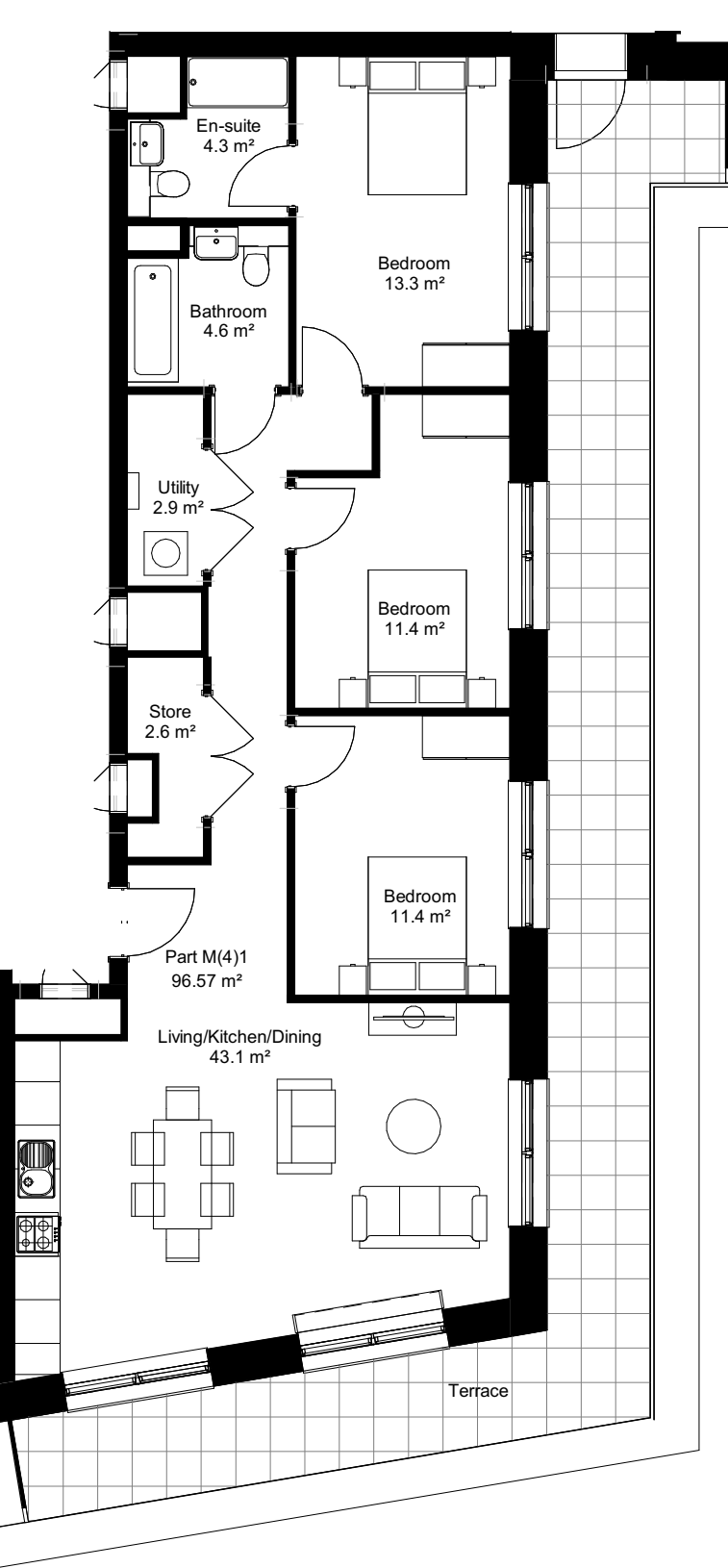
Level 7 KEY PLAN FLAT 17_Planning 1 : 1000
