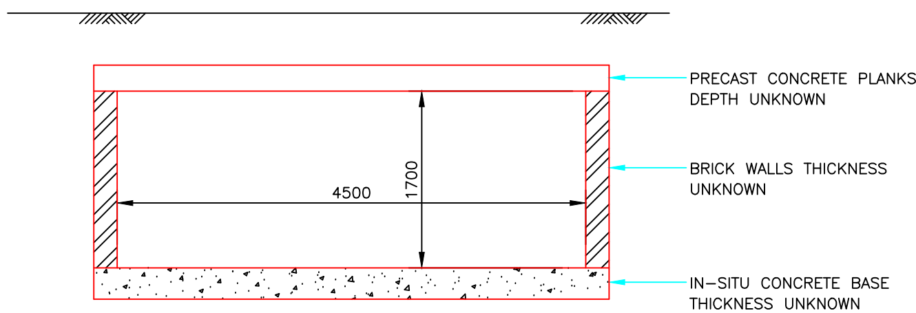
SECTION AT CHAINAGE 220
