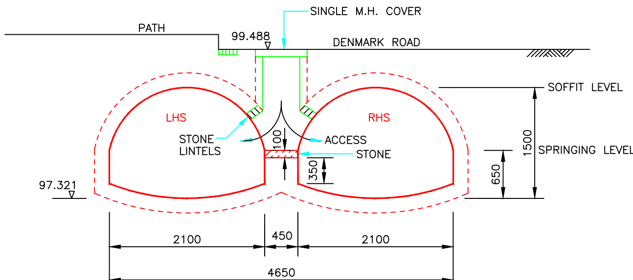
TWIN CULVERT - SECTION AT ACCESS DRC 2, CHAINAGE 0
