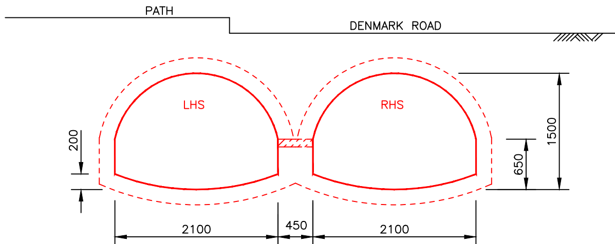
TYPICAL SECTION THROUGH BRICK CULVERT
