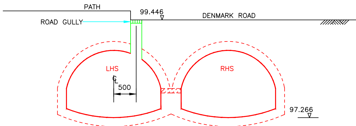
SECTION AT CHAINAGE 70
