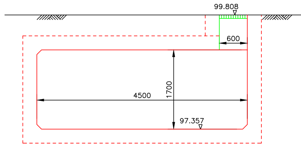
SECTION AT CHAINAGE 194
