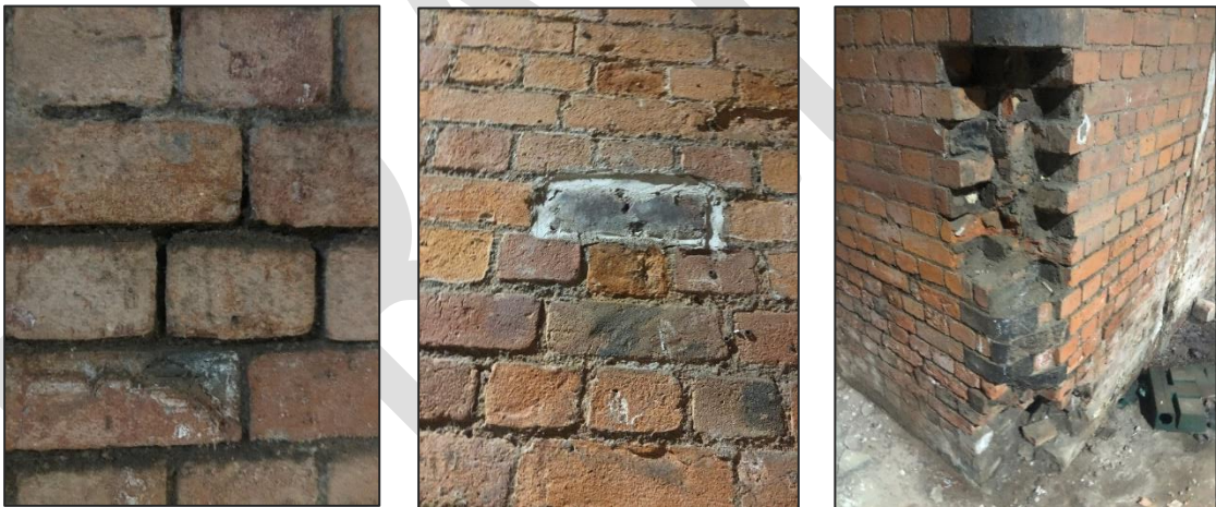
Figure 8 (left): Example of internal brickwork where lime mortar infill would be required. Figure 9 (centre): Example of concrete mortar infill to be carefully removed and repaired. Figure 10: example of missing brickwork (blue brick) needed to be replaced like-for-like.
