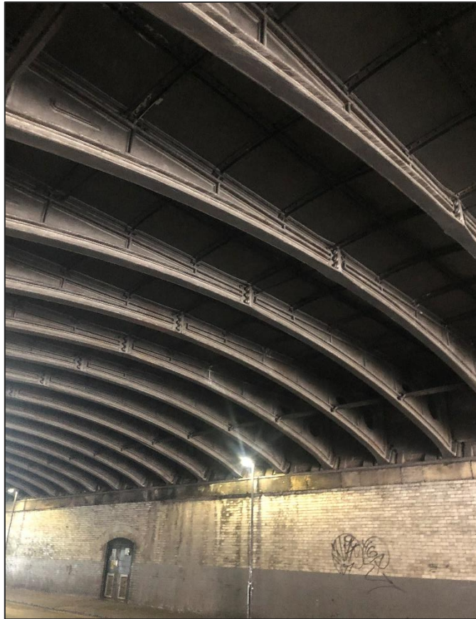
Figure 5: Photo of the underside of the cast iron bridge to Great Bridgewater Street.
