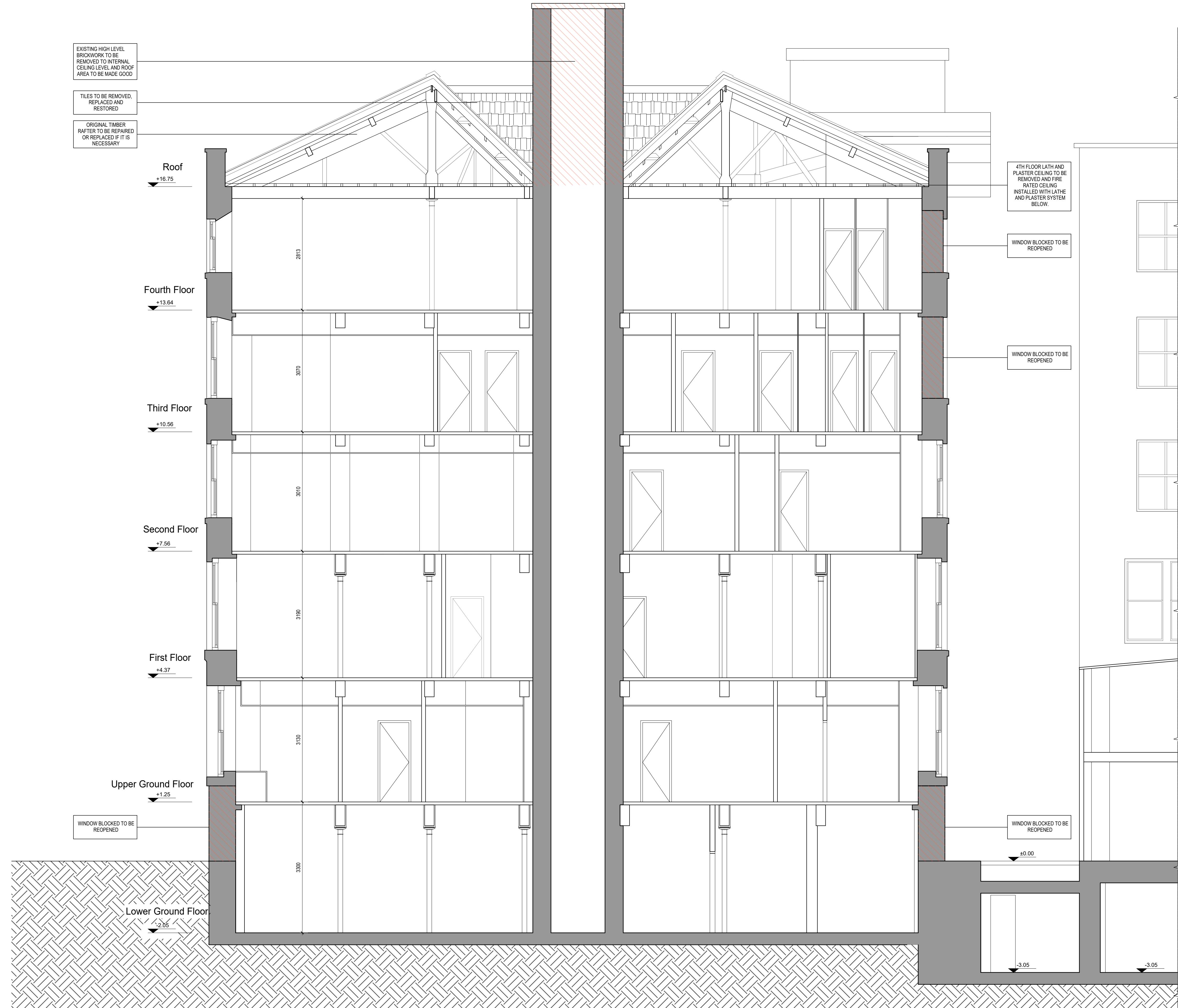
Existing Section A-A
