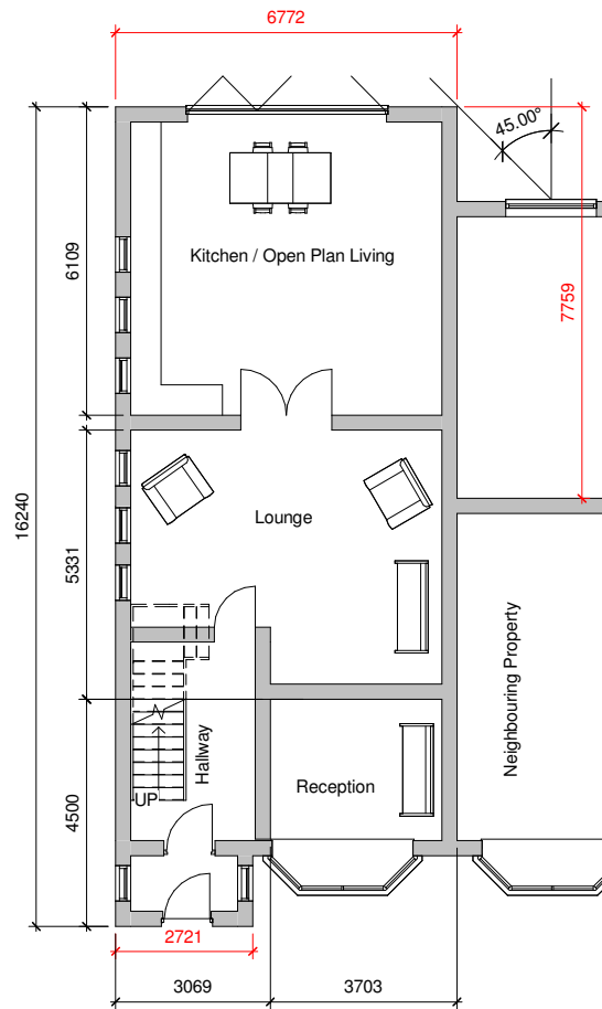
1 Ground Floor 1 : 100
