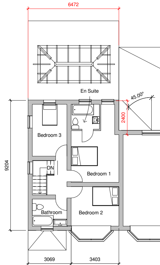
2 First Floor 1 : 100
