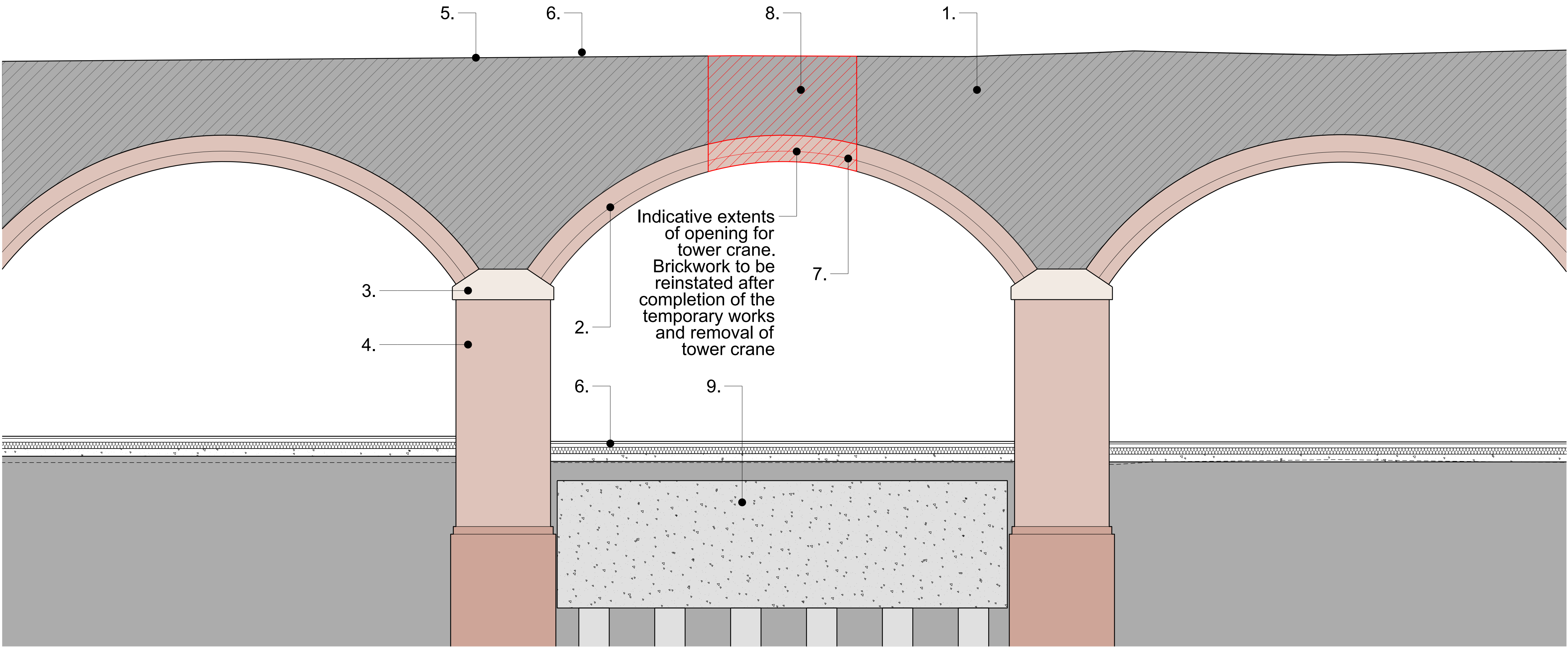
Proposed Detailed Section Through the Viaduct
