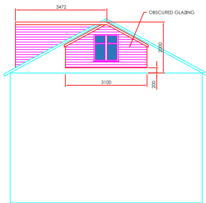
PROPOSED SIDE ELEVATION
