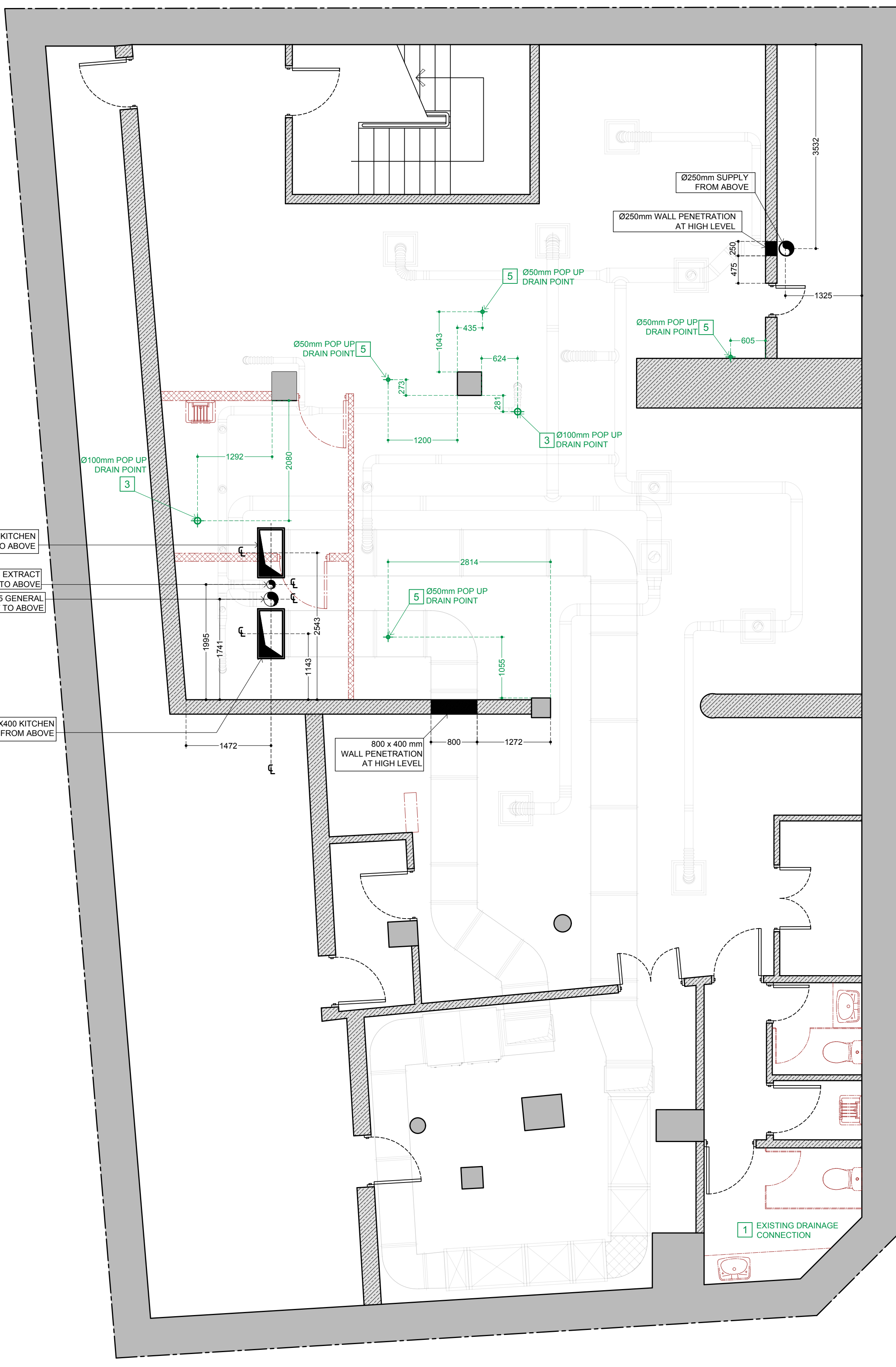
01 BASEMENT SCALE 1:50 @ A1
