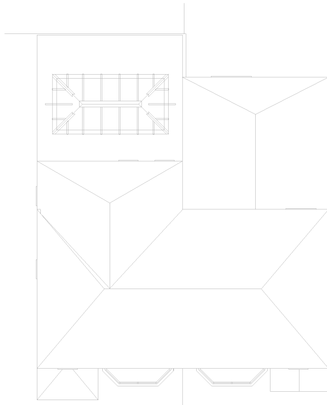
1 Proposed Roof Plan 1 : 100
