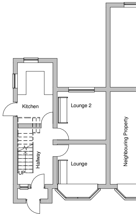
1 Ground Floor 1 : 100
