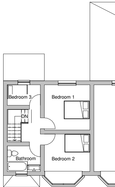
2 First Floor 1 : 100
