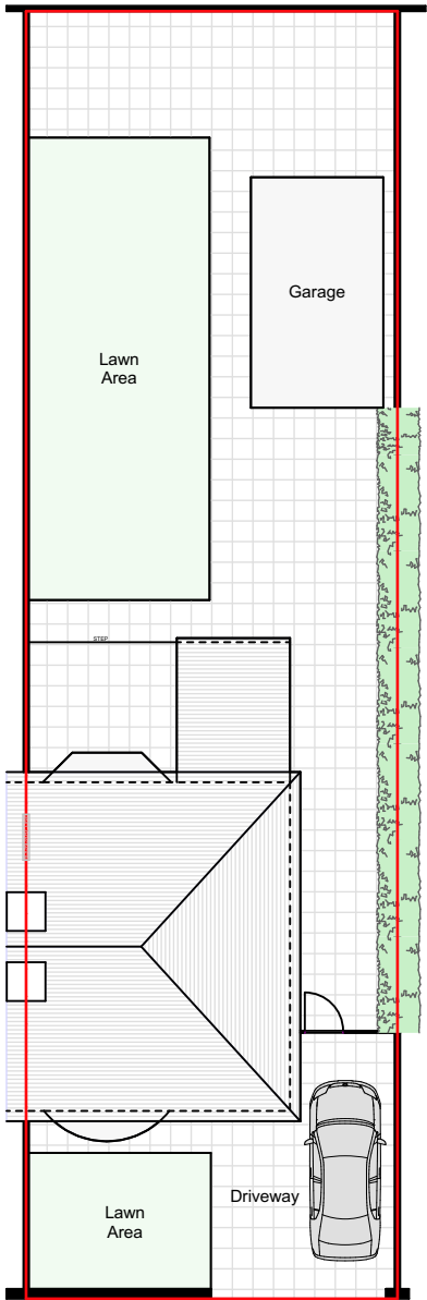
EXISTING GA SITE PLAN @1:200
