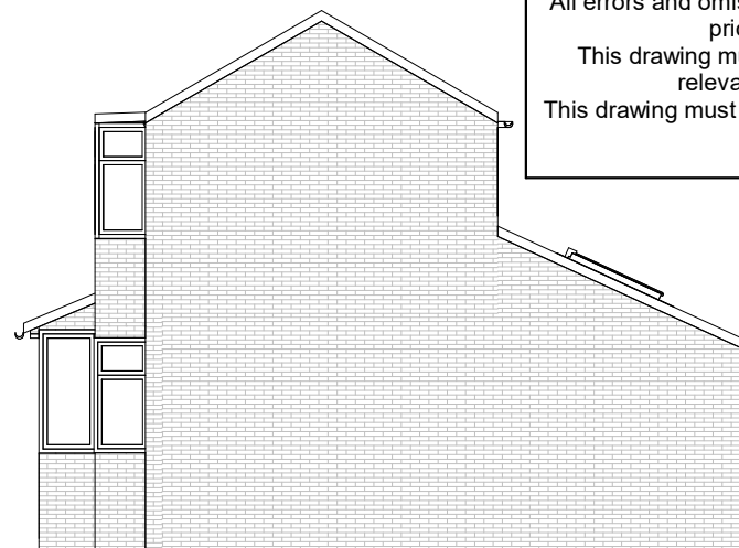
2 Left Proposed
