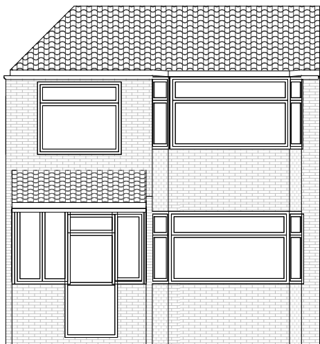
1 Front Proposed
