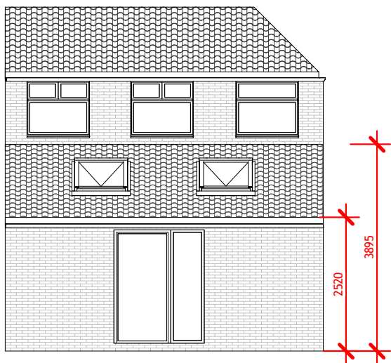
3 Rear Proposed
