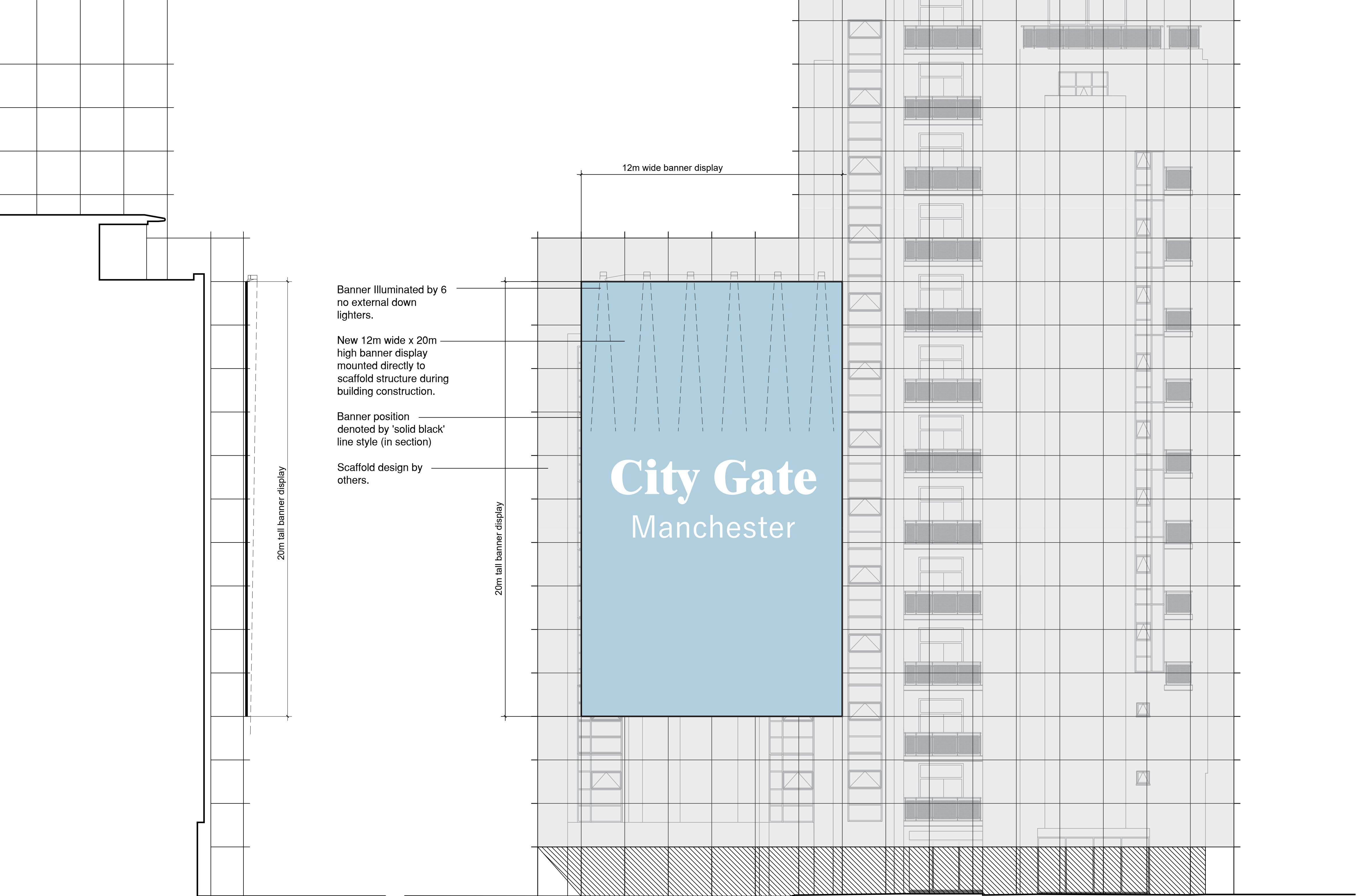
Typical Section Through (as Proposed)
