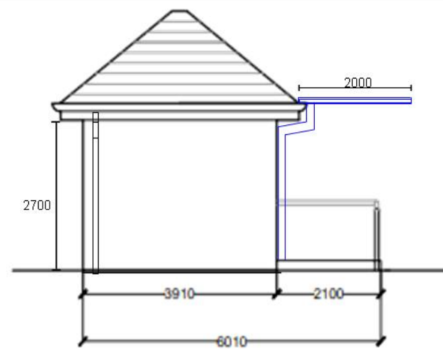
SIDE ELEVATION (LEFT) 1:100
