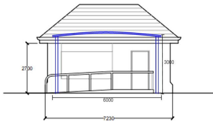
FRONT ELEVATION 1:100
