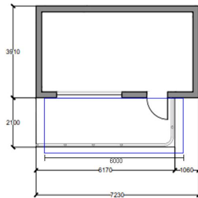
GF PLAN 1:100
