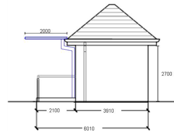
SIDE ELEVATION (RIGHT) 1:100
