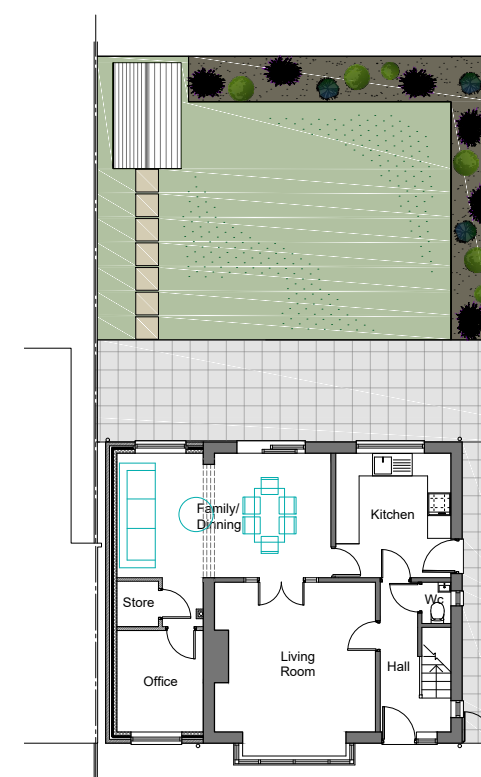
PROPOSED GROUND FLOOR PLAN IN CONTEXT
