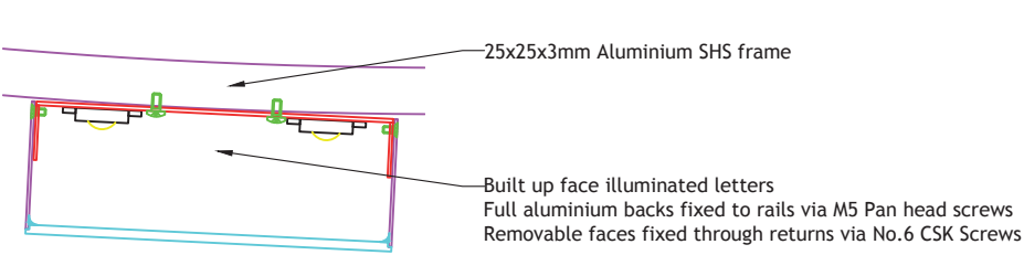
Detail B 1:4 @ A3
