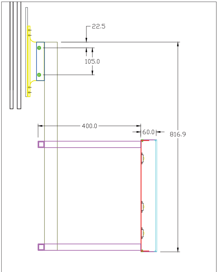
Side view (1:8 @ A3)
