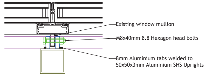
Detail A 1:4 @ A3
