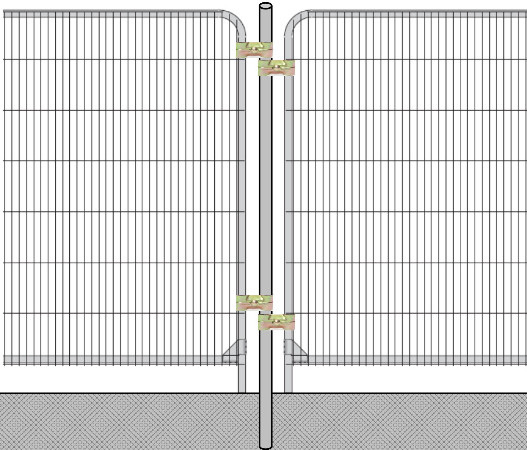
FENCING INSTALLED VIA SCAFFOLD TUBE CONCRETED BETWEEN PANELS
