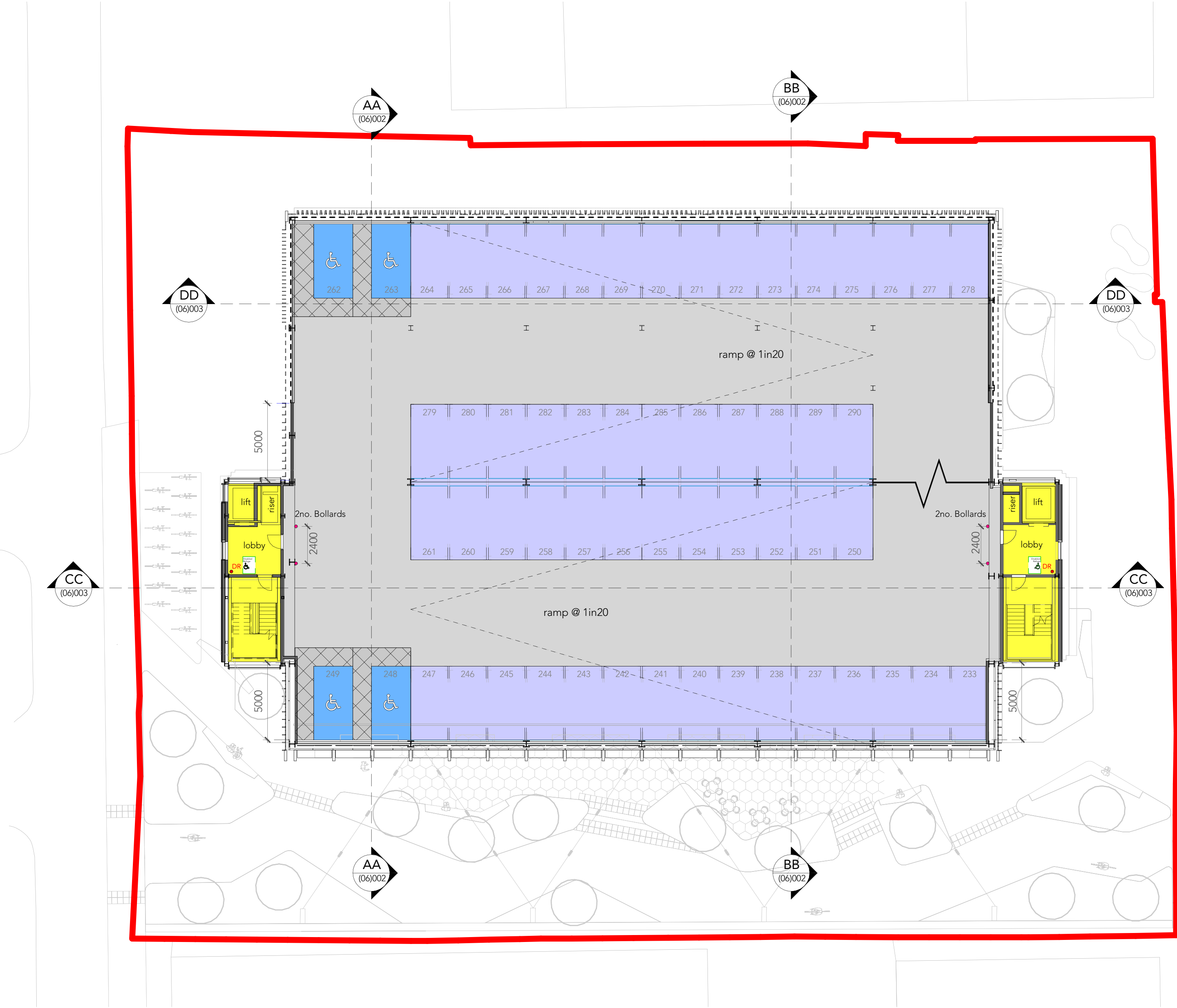
Fifth Floor GA Plan
