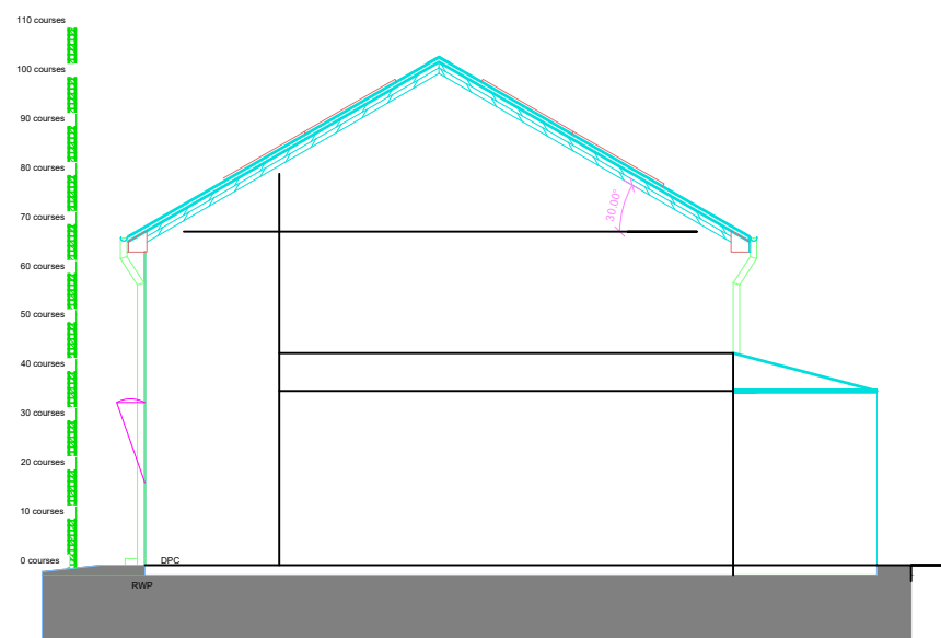
4 Proposed Side B Elevation 1 : 50
