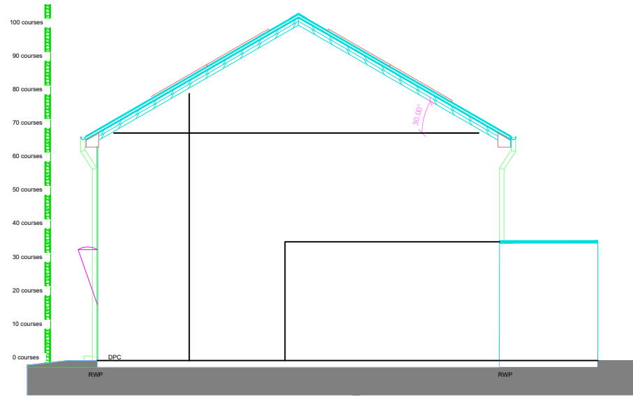
3 Existing Side B Elevation 1 : 50
