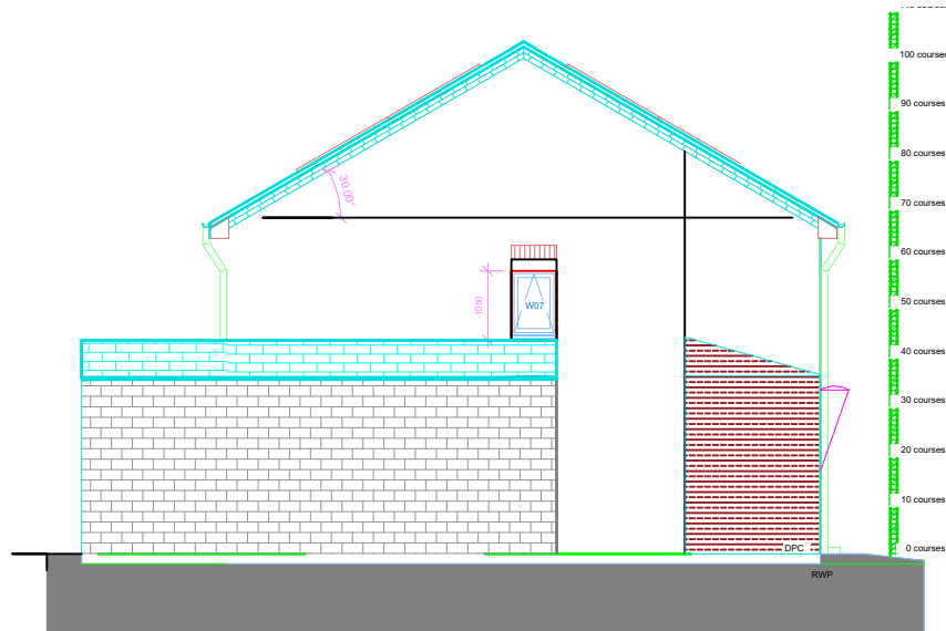
1 Existing Side A Elevation 1 : 50
