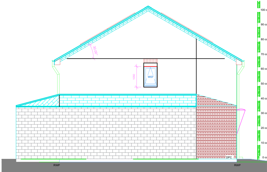
2 Proposed Side A Elevation 1 : 50
