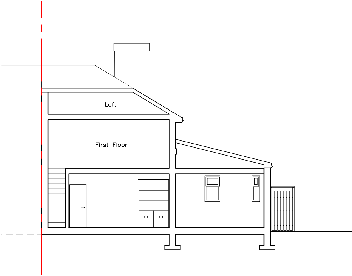
Proposed Section
