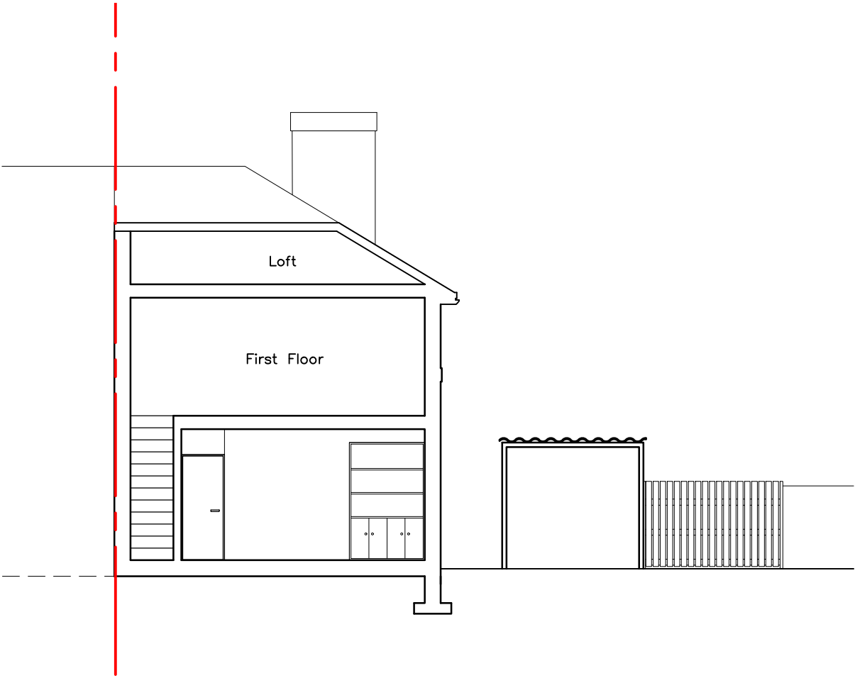
Existing Section
