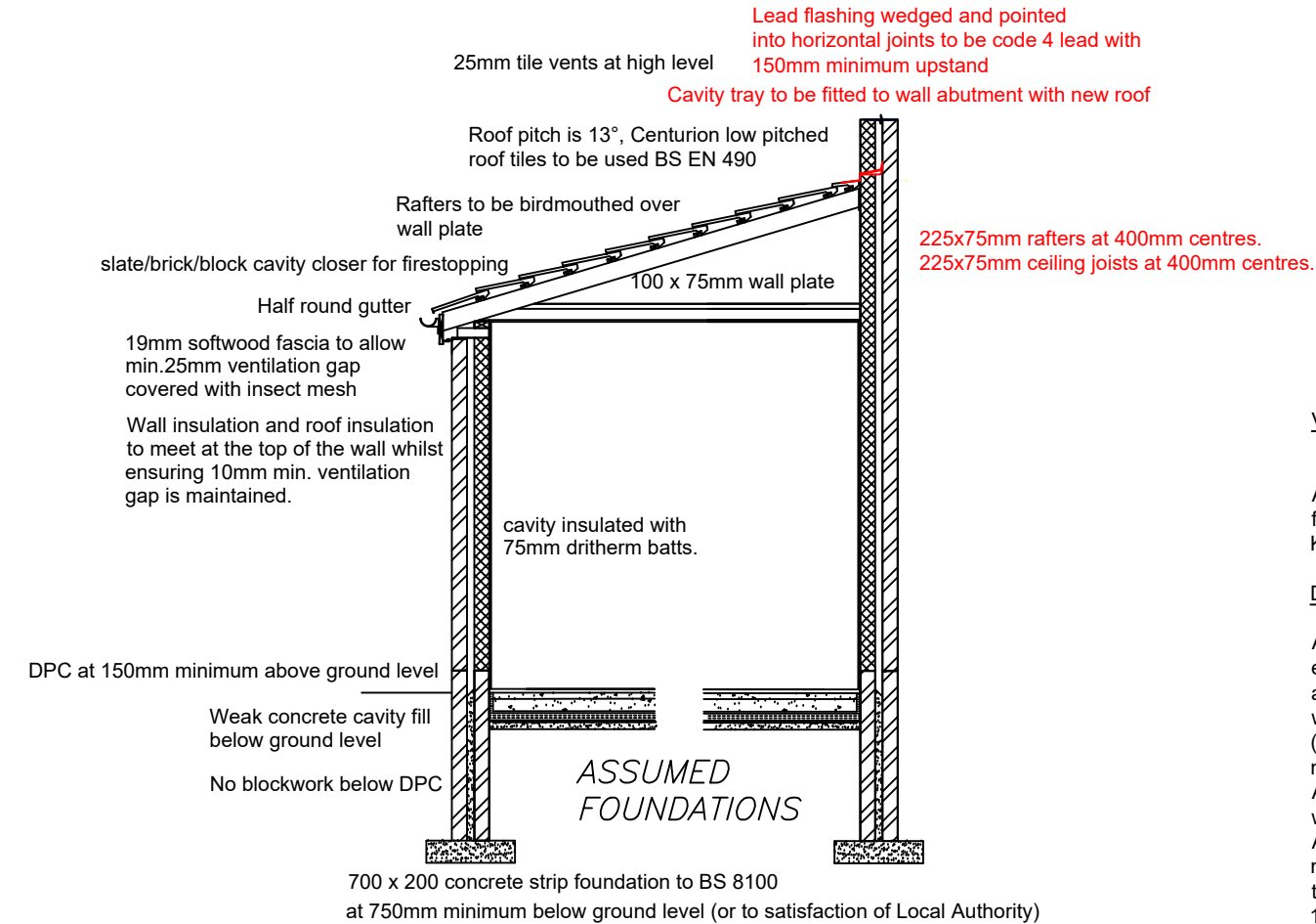
TYPICAL SECTION
