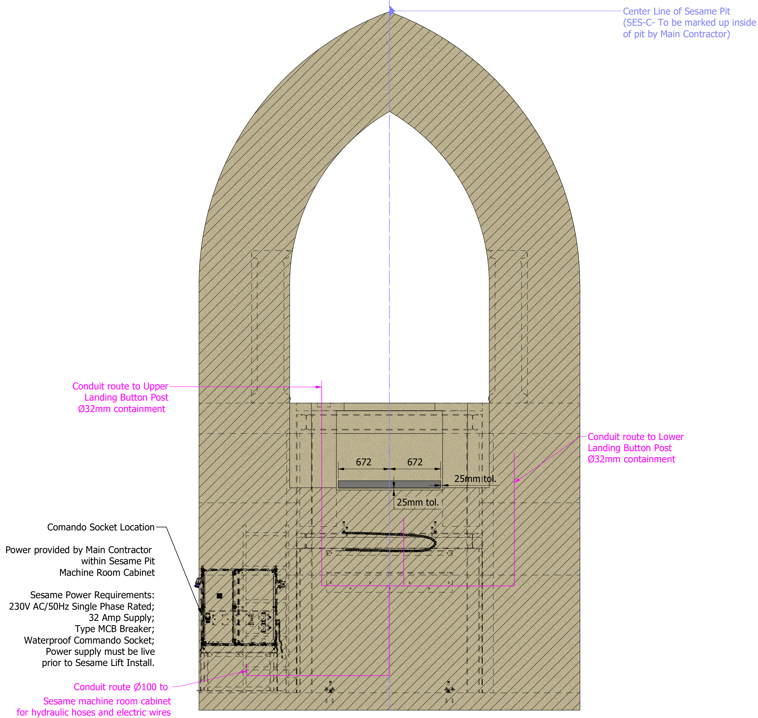
F-F ( 1:30 )
