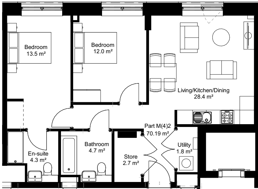
Level 1 KEY PLAN FLAT 10_Planning 1 : 1000
