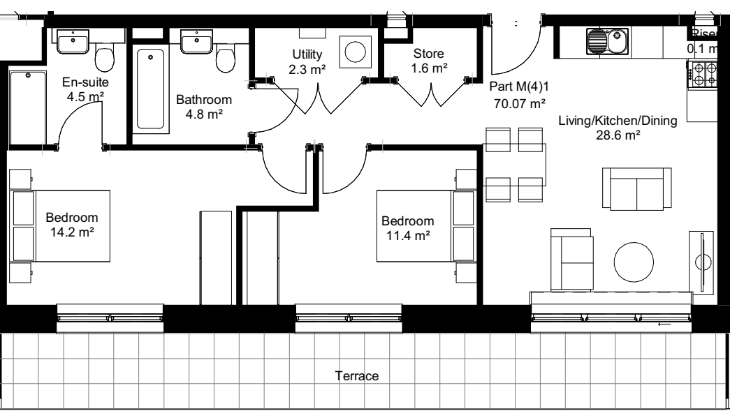
Level 7 KEY PLAN FLAT 9_Planning 1 : 1000
