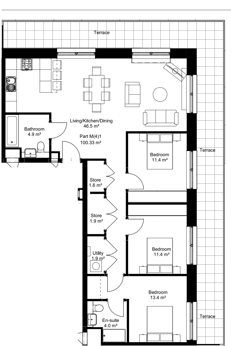
Level 7 KEY PLAN FLAT 13_Planning 1 : 1000
