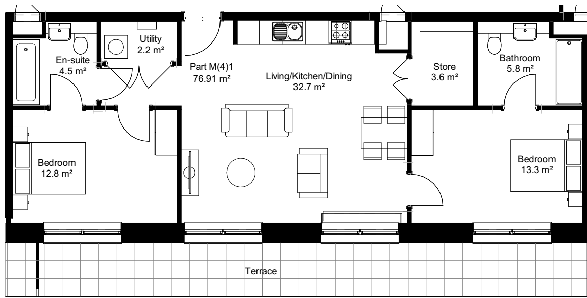
Level 7 KEY PLAN FLAT 11_Planning 1 : 1000
