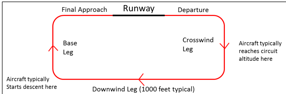
Figure 7 – Typical circuit diagram
