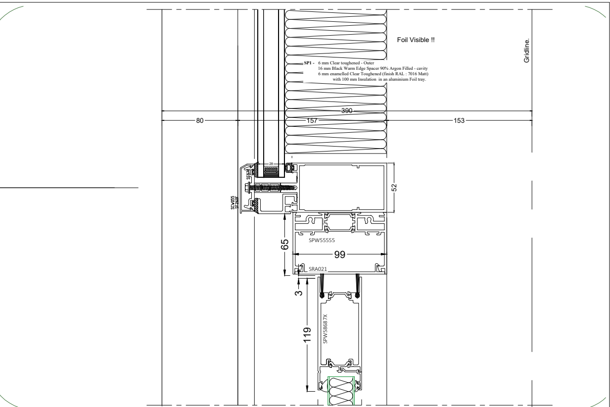
02 Typical Curtainwall Door Head Detail (CW-09). Scale: 1:2
