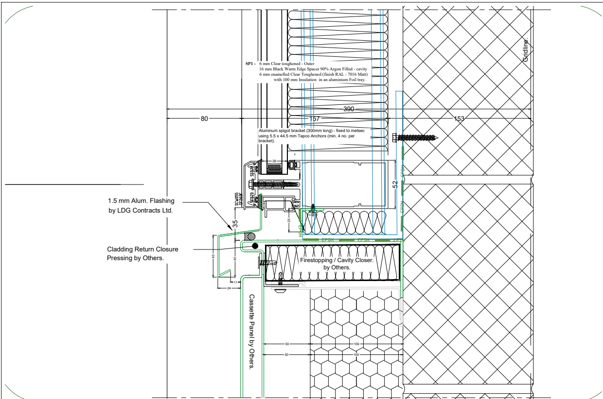
04 Typical Curtainwall Cill Detail above Cladding. Scale: 1:2
