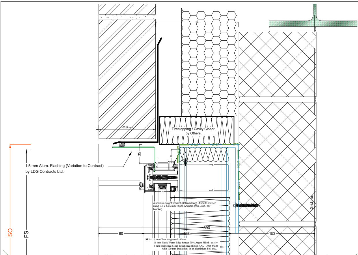
03 Proposed Curtainwall Head Detail above Cladding. Scale: 1:2
