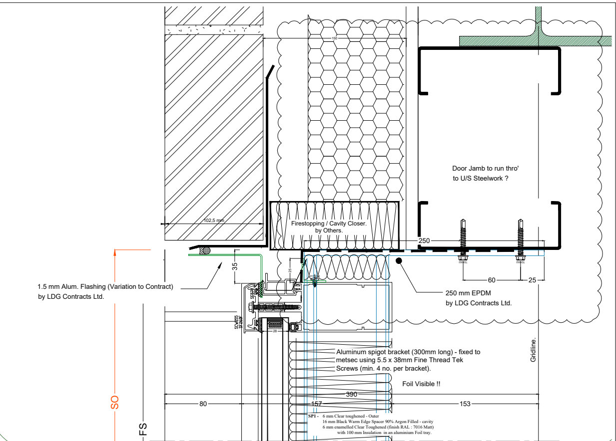
01 Proposed Curtainwall Head Detail above door (CW-09). Scale: 1:2
