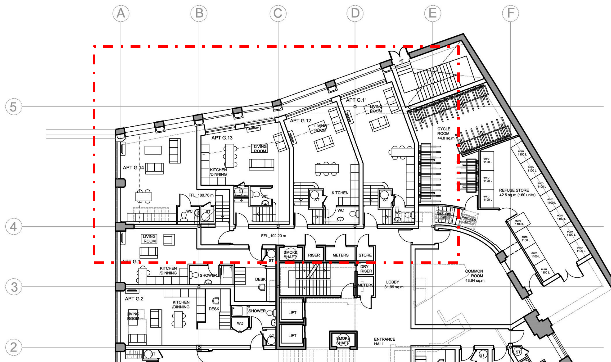
Above is an extract from the proposed ground floor plan showing the proposed apartments G11, G12, G13 & G14 created by converting the former car park
